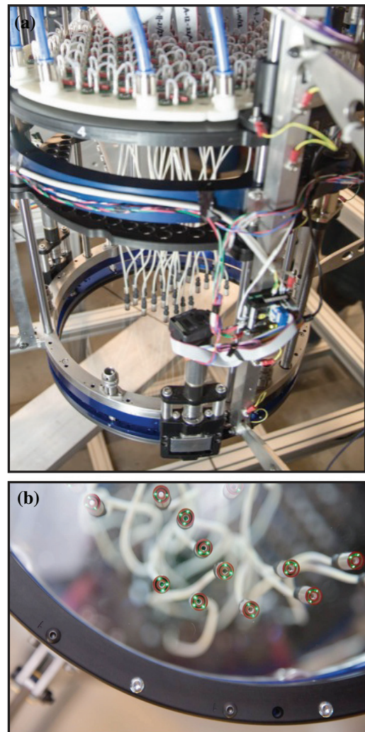
Figure 1. The TAI PAN fibre positioner at the AAO. (a) Top view, showing 24 Starbugs installed on the glass field plate that sits at the focal surface of the UKST. The top of the image shows the complex vacuum and high-voltage support systems required for operation. (b) Underside view, showing some of the 24 Starbugs installed on the glass field plate.
