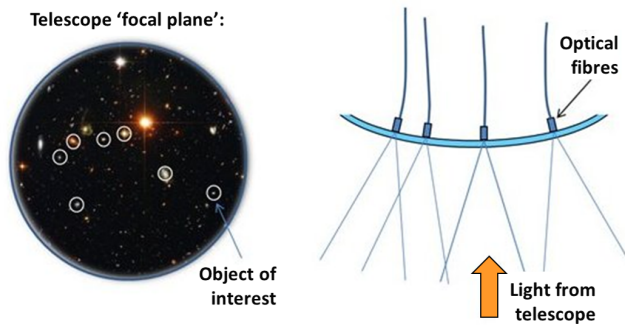
Figure 2. Schematic representation of the TAIPAN focal plane. The background image shows target galaxies as ‘objects of interest’, while Starbugs are the depicted by the white open circles. Starbugs can move independently to put a spectroscopic fibre on any object of interest in the 6-degree diameter field of view. The right-hand side shows a side view.
