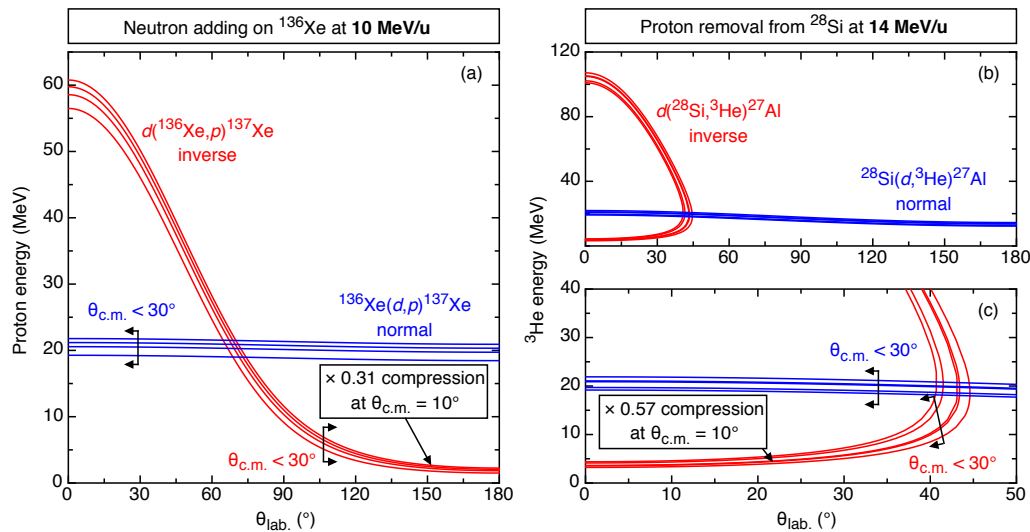
Figure 1. (Colour online) (a) Kinematic lines of proton energy versus \theta_{\text{lab.}} for the d(^{136}\text{Xe},p)^{137}\text{Xe} reaction at 10 MeV/u following population of the 0, 601, 1218, and 2510-keV states in ^{137}\text{Xe} in both normal (blue) and inverse (red) kinematics. (b) Similar lines for ^3\text{He} ions following population of the 0, 884, 1015, 2212, and 2735-keV states in ^{27}\text{Al} via the d(^{28}\text{Si},^3\text{He})^{27}\text{Al} reaction at 14 MeV/u, with (c) focussing on the forward centre-of-mass angles to emphasise the two-solution nature of negative Q value reactions in inverse kinematics.
