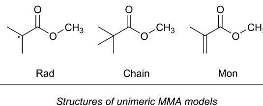
Fig. 4 Unimeric models of the MMA polymer terminus (Rad), polymer chain (Chain) and the structure of MMA monomer (Mon).
