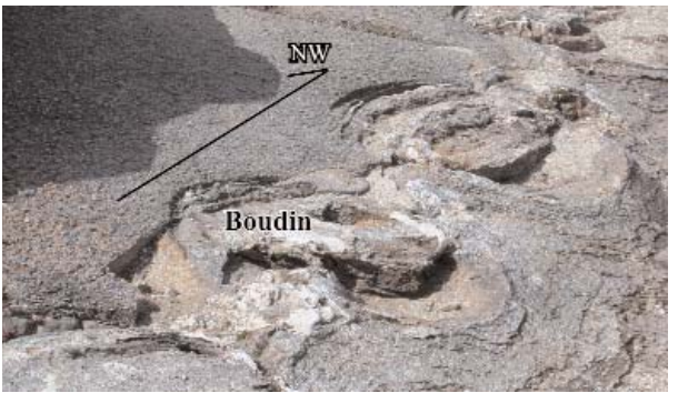
Fig. 16 - Foliation boudinage in the quartz-rich metasediment. Abundant garnets are found immediately below the overlying tectonic contact with the Zermatt Saas Zone. The trend of the boudinage is NW/SE, parallel to the dominant stretching lineation. FOV ~4m. (E:0390724 N: 5081418).
