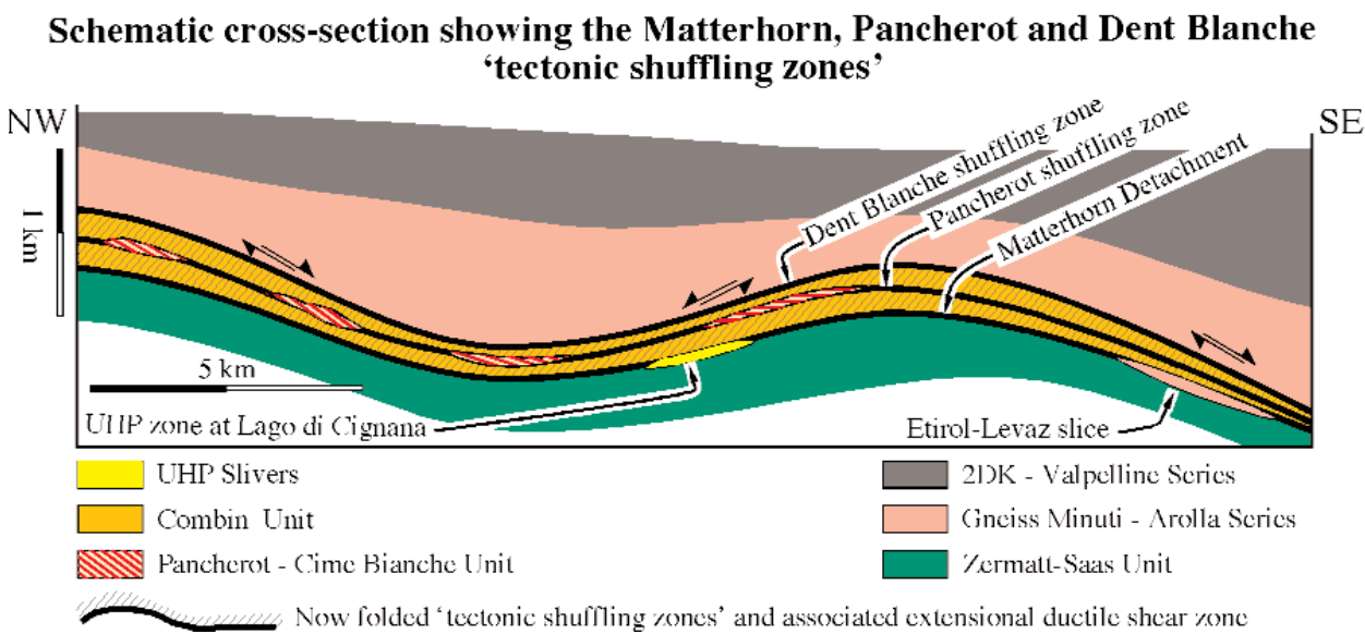
Fig. 6 - The diagram shows structural relations as would have applied at the end of the extensional phase (at ca 36 Ma). Post ca 25 Ma the Alpine crust was folded to produce the present geometry (as shown in Fig. 3). The base of the extensional shear zone that affected the Combin Zone is cut off by the semi-brittle Matterhorn Detachment. A similar fault may exist at the Dent Blanche contact, where a narrow more intense shear zone is also observed. Tectonic shuffling zones may be the result of thrusts that have been re-activated as detachment faults/shear zones, stranding anastomosing lenses of higher pressure rocks. Crustal-scale boudinage during the later stages of movement may have overprinted adjacent parts of the shear zone differently, producing shear sense variation as shown. The shear zones at Lago di Cignana were affected by NW-directed sense of shear at this time, while zones to the southeast (e.g. Gressoney) were affected by SE-directed sense of shear (REDDY et alii 2003).
