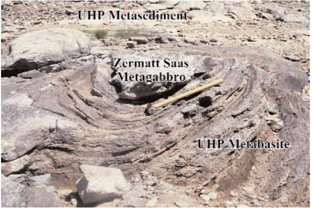
Fig. 18 - Zermatt Saas Fe-Ti metagabbro overlying UHP metabasites. Shearing is most intense immediately adjacent to this tectonic contact. A late-stage, NW/SE compressional event has caused metre-scale folding, here downwarping the overlying Zermatt Saas metagabbro sheet.
