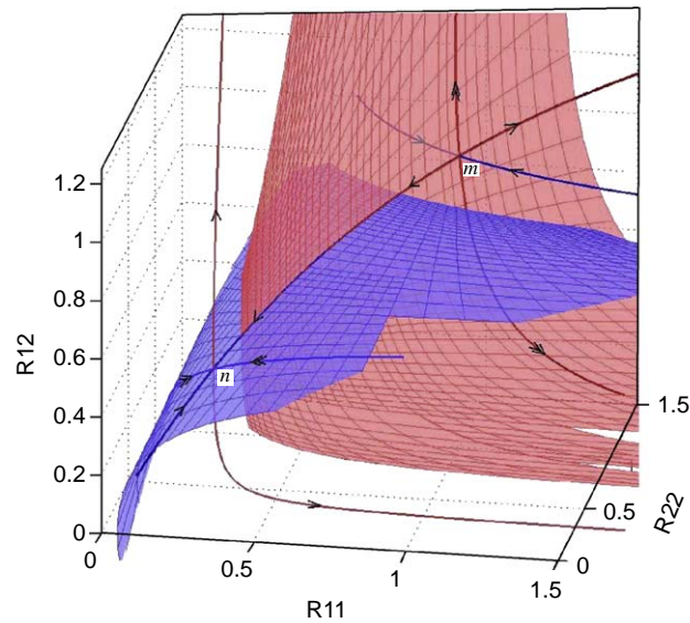
Fig. 1. Invariant manifolds of the ABS model.
