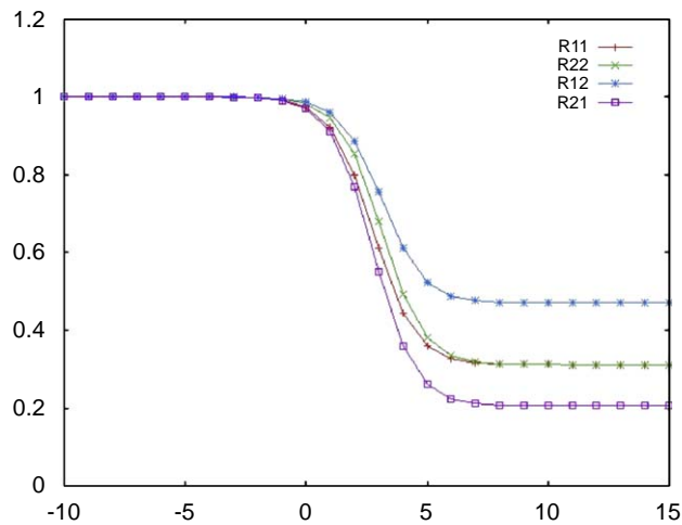
Fig. 2. Time series of the rates of return of an heteroclinic point.
