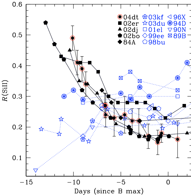
Fig. 12. Premaximum temporal evolution of the R(\text{Si II}) parameter for SN 2004dt and a sample of SNe shown for comparison. Filled symbols refer to HVG SNe, open symbols to LVG SNe, as defined in Benetti et al. (2005).
