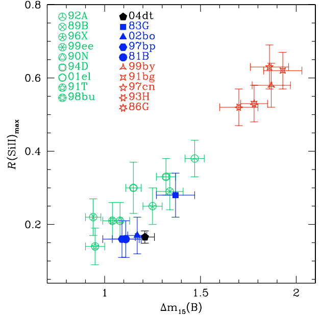
Fig. 10. R(\text{Si II}) vs. \Delta m_{15}B for SN 2004dt and a sample of SNe shown for comparison. Filled symbols refer to HVG SNe, starred symbols to FAINT SNe, and all the others to LVG SNe, as defined in Benetti et al. (2005).
