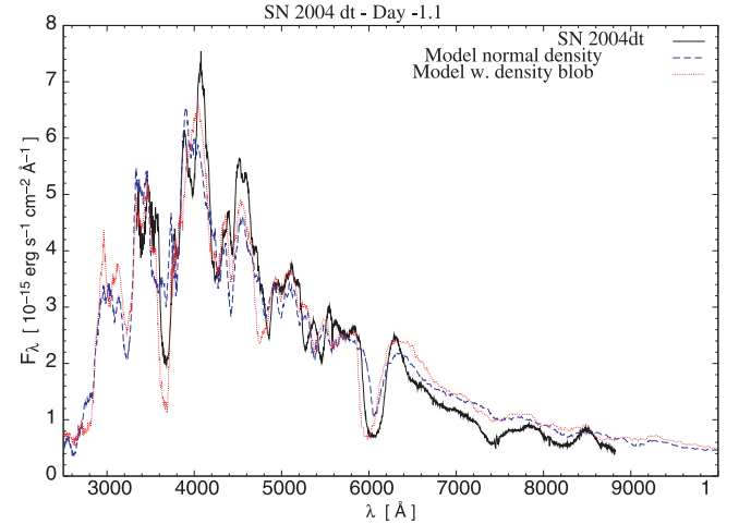
Fig. 15. Observed spectrum and corresponding model of SN 2004dt at day -1.1 using E(B - V) = 0.0 , \mu = 34.61 , t_{\text{exp}} = 17.7 d.
