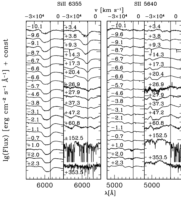
Fig. 7. Evolution with time of the Si II \lambda 6355 Å (left panel) and S II \lambda 5454, 5640 Å (right panel). Vertical lines at 6150 and 5500 Å are shown to guide the eye.
