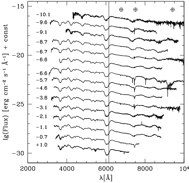
Fig. 2. Early spectral sequence for SN 2004dt. The vertical line at \lambda = 6150 Å makes the evolution of the blueshifted Si II \lambda 6355 Å feature clear. Spectra are restframe. No reddening correction has been applied. The \oplus symbols mark the position of the main telluric absorptions, which have been partially removed. Spectra have been shifted downwards for clarity (shift step = -1). The phase with respect to the maximum of the B light curve is shown to the left of each spectrum.
