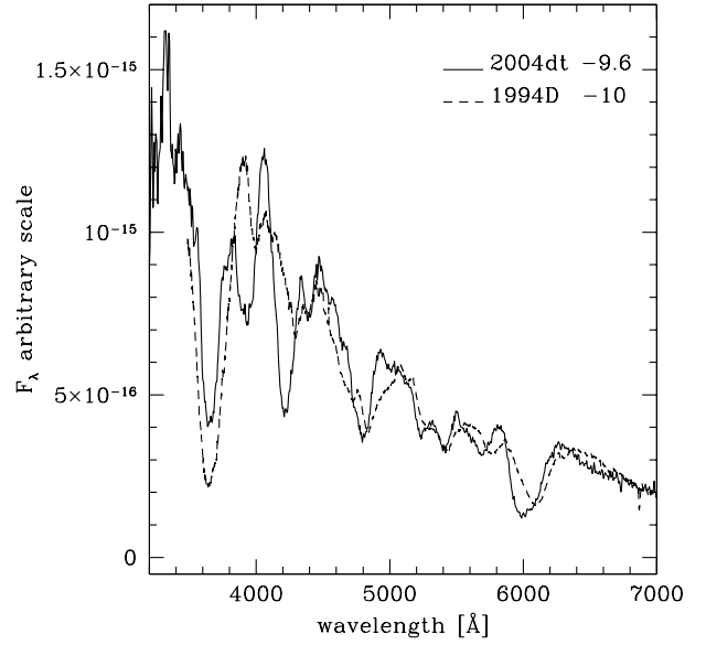
Fig. 4. Comparison among spectra of SN 2004dt (solid line) and SN 1994D (dashed line) \sim 10 days before maximum. To be noticed the very different blue-shift of the Si II \lambda 6355 Å features and the more similar blue-shift of the Si II \lambda 5960 Å lines. Significant differences are present in the 3800 – 4200 Å region.
