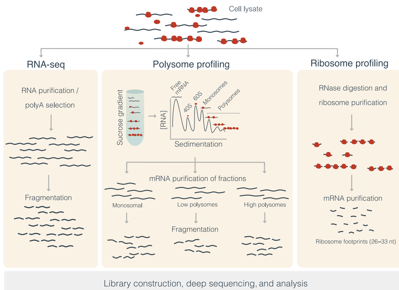
FIGURE 3 High-throughput approaches to capture the translome. RNA sequencing can capture all mRNAs in the cell lysate regardless of its translation status (left panel). Polysome profiling (middle panel) separates fractions of mRNAs according to the number of ribosomes attached to the mRNAs, which is assumed to correlate with the translation activity. Downstream sequencing of RNA in each polysomal fraction is performed as a standard RNA-seq experiment, and the relative mRNAs abundances are interpreted as mRNA translation activities. In ribosome profiling or Ribo-seq (right panel), mRNAs bound by the ribosomes are digested, producing footprints of approximately 30 nt representing the mRNA sites occupied by the ribosome. These fragments are then sequenced after detaching the ribosomes
