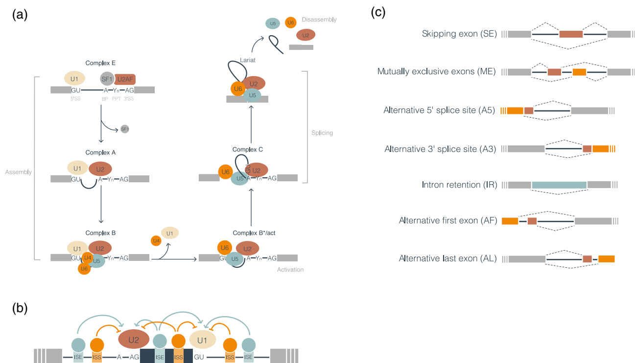
FIGURE 1 The mechanisms of splicing and alternative splicing. (a) The complexes and processing steps of splicing for the major spliceosome are depicted. In the assembly phase, U1, U2, U4, U5, and U6 are sequentially assembled in the mRNA molecule resulting in the formation of complex E, complex A, and finally, complex B. The activation phase consists of conformational and compositional rearrangements of complex B involving U2, U5, and U6. Two transesterifications occur as the catalytic complex C adapts its conformation: the first between the 5' SS and the BP and the second between the 5' end of the first exon and the 3' end of the second exon. Finally, the snRNPs still attached to the mRNA disassemble to start a new cycle. (b) Illustration of the regulation of splicing by cis - and trans -acting factors. Cis -acting factors are represented as boxes in introns and exons. Trans -acting factors are represented as circles bound to their corresponding cis -acting elements: exonic splicing enhancer (ESE), exonic splicing silencer (ESS), intronic splicing enhancer (ISE), or intronic splicing silencer (ISS). Silencers are depicted in orange and enhancers in light blue. (c) Schematic representation of alternative splicing events. Gray boxes represent constitutive exons, red and orange boxes represent alternative exons, and a light blue box represents an exonized intron. Discontinuous ends in the exons indicate that the transcript continues in that direction. Thick blue lines represent introns in the transcript before processing, and dashed lines above and below represent the alternative processing of the exons
