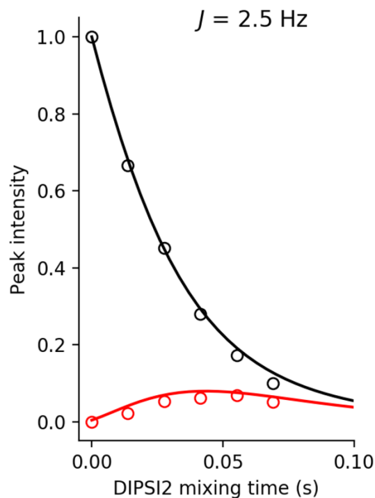
Figure S9. Diagonal and cross-peak intensities in ^{19}\text{F} - ^{19}\text{F} TOCSY spectra as a function of mixing time. Data were simulated using the program Spinach for two \text{CF}_3 groups as detailed in the experimental section. 17 The simulations applied DIPSI2 mixing to longitudinal magnetization, followed by an excitation pulse. To alleviate antiphase dispersive components, the peak heights were monitored after apodization with a 50 Hz exponential window function. Experimentally measured data of PpiB \text{CF}_3 -Tyr(27,98) are shown as open circles. The experimental data were scaled by setting the diagonal peak height at zero mixing time to one. Black and red lines indicate the diagonal and cross-peak heights, respectively.
