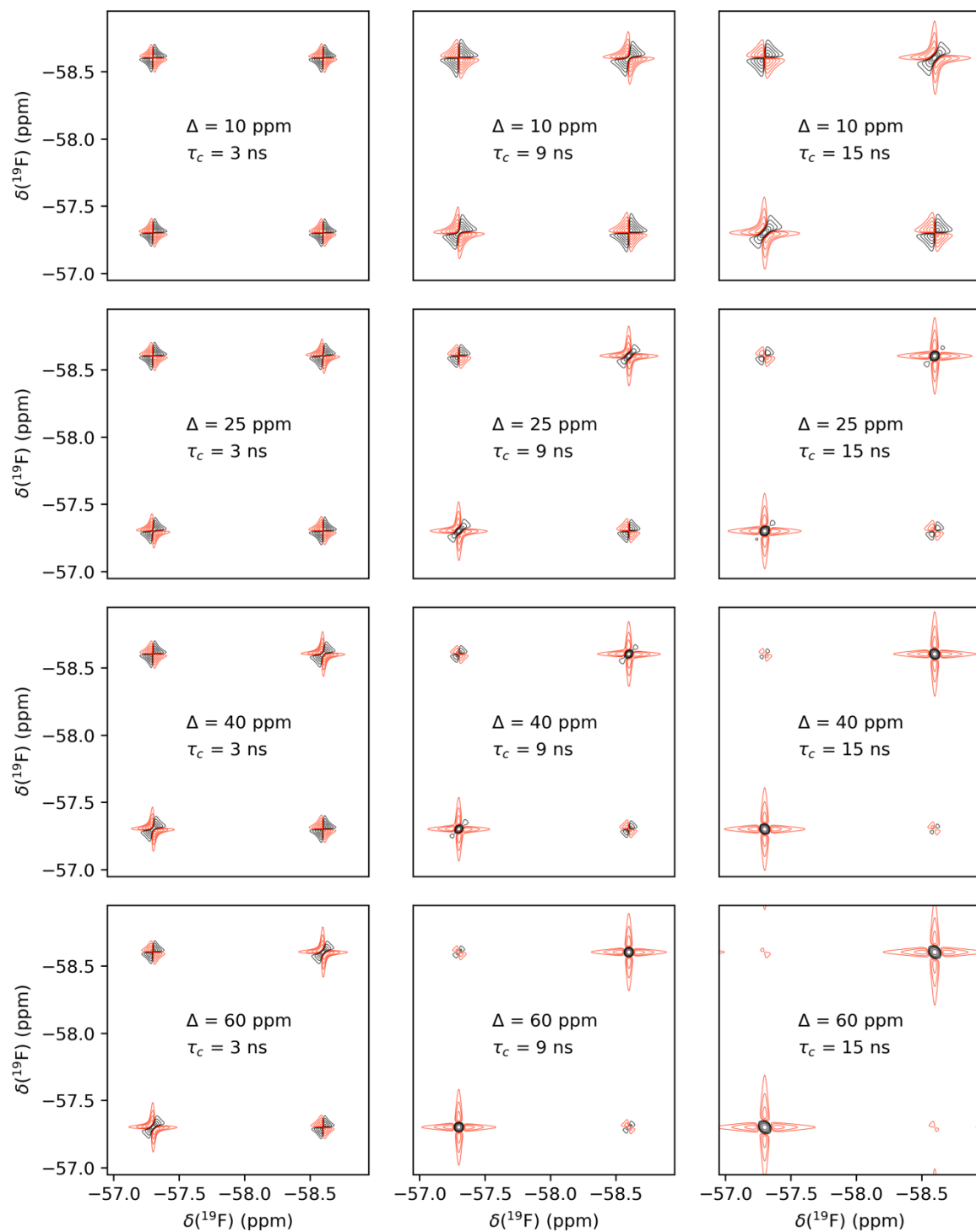
Figure S11. ^{19}\text{F} - ^{19}\text{F} DQF-COSY spectra of PpiB CF 3 -Tyr(27,98) simulated using the program Spinach with ^{\text{TS}}J_{\text{FF}} = 2.5 Hz. 17 Each spectrum was calculated for a given CSA tensor anisotropy \Delta and rotational correlation time \tau_c as shown. All spectra were plotted with the lowest contour level set at 1.7% of the height of the diagonal peak and using a factor of 2 between subsequent contour levels.
