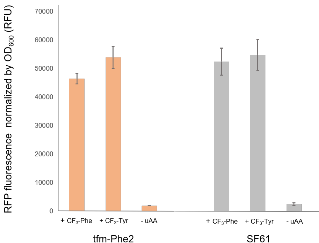
Figure S1. RFP fluorescence levels normalized by OD 600 in cell cultures producing RFP with CF 3 -Phe or CF 3 -Tyr incorporated by amber codon read-through by tfm-Phe2 or SF61. Error bars were derived from six biological replicates. SF61 is an aminoacyl-tRNA synthetase selected for incorporation of SF 5 -Phe into proteins. 3 Its ready recognition of CF 3 -Phe and CF 3 -Tyr demonstrates multi-specificity.
