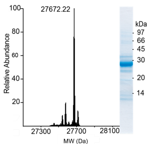
Figure S13. Mass spectrum and SDS-PAGE of AncCDT-1 TFA-Lys(68,162). The calculated mass is 27,673.67 Da. The second largest peak in the mass spectrum corresponds to a glutamine mis-incorporated in place of a TFA-Lys residue (experimental mass: 27,576.17 Da, calculated: 27,577.61 Da).
