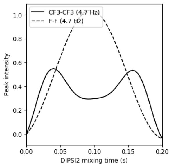
Figure S10. Cross-peak intensities relative to the diagonal peak intensities in ^{19}\text{F} – ^{19}\text{F} TOCSY spectra as a function of DIPSI2 mixing time and in the absence of relaxation. Data simulated using the program Spinach. 17 Solid and dashed curves show the results for J_{\text{FF}} couplings between two \text{CF}_3 groups and two single ^{19}\text{F} spins, respectively, with a coupling constant of 4.7 Hz.
