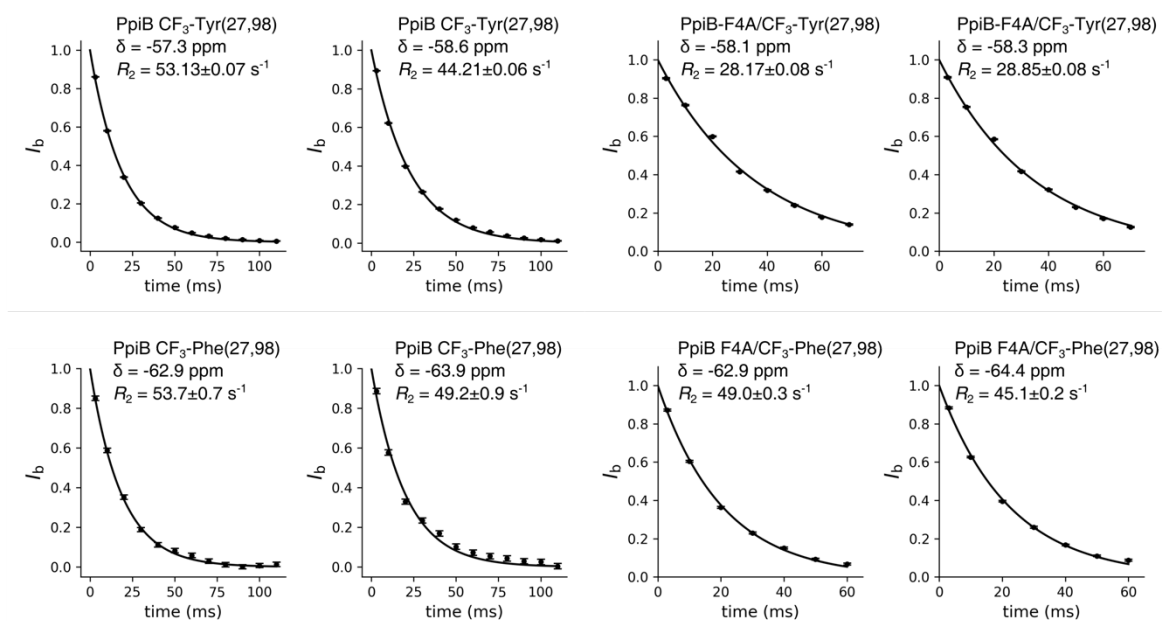
Figure S7. Decay of transverse ^{19}\text{F} magnetization in different \text{CF}_3 mutants of PpiB determined from fitting the data measured in the quantitative J evolution reference experiment. The ^{19}\text{F} chemical shifts and transverse relaxation rates are indicated in the plots.
