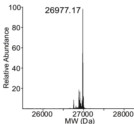
Figure S14. Mass spectrum of mRFP TFA-Lys(192,225). The calculated mass (following loss of the N-terminal methionine) is 26,978.28 Da. The second largest peak in the mass spectrum corresponds to a glutamine mis-incorporated in place of a TFA-Lys residue (experimental mass: 26882.17 Da, calculated: 26,882.23 Da).
