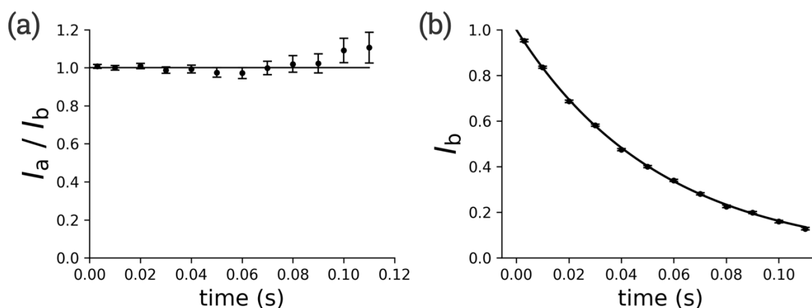
Figure S5. Control experiment of the quantitative J evolution experiment of Figures 7 and 8 conducted with a protein containing a single fluorine, GB1 with Trp43 replaced by 7-fluorotryptophan. (a) Relative peak intensities observed in experiments a and b of Figure 7 plotted versus the spin echo delay \tau . (b) Decay of the signal in experiment b of Figure 7. The fit determined the transverse relaxation rate R_2 as 18.5 \pm 0.07 \text{ s}^{-1} .
