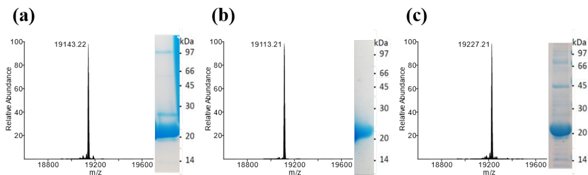
Figure S2. Mass spectra and SDS-PAGE of PpiB mutants with CF 3 -Tyr or CF 3 -Phe residues. (a) PpiB CF 3 -Tyr(27,98); calculated mass 19,144.36 Da. (b) PpiB CF 3 -Phe(27,98); calculated mass 19112.36 Da. (c) PpiB CF 3 -Tyr(4,27,98); calculated mass 19,228.36 Da.
