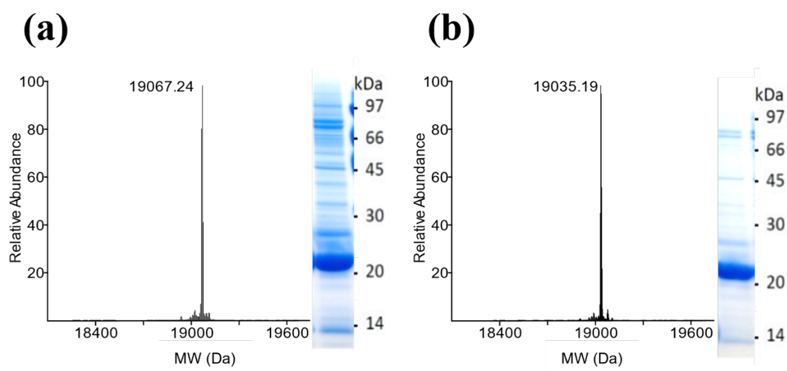
Figure S3. Mass spectra and SDS-PAGE of PpiB Phe4Ala mutants with CF 3 -Tyr or CF 3 -Phe residues. (a) PpiB F4A/CF 3 -Tyr (27,98); calculated mass 19,068.26 Da. (b) PpiB F4A/CF 3 -Phe (27,98); calculated mass 19,036.26 Da.
