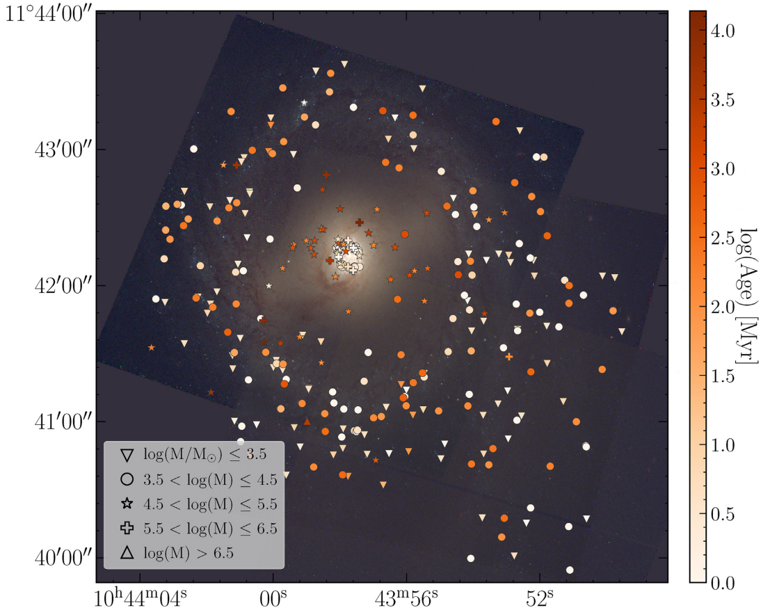
Figure 10. Colour image of NGC 3351 with the location of the clusters overplotted. Clusters are colour-coded by best-fitting \log(\text{Age}/\text{Myr}) . Data point symbols differentiate between five \log(\text{Mass}/M_{\odot}) bins. The majority of clusters found in the outer ring and disc fall in the two lowest mass bins (downward triangles and circles). Higher mass clusters (stars and crosses) are generally found to be in the stellar bulge and the inner star-forming ring. The most massive cluster (upward triangle) is located in the outer ring.
