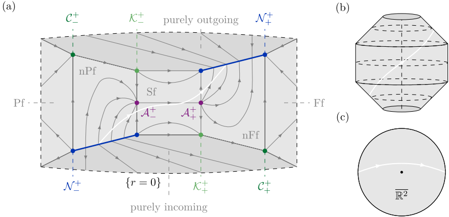
Fig. 3. a The flow, for g the Minkowski metric, in the subset of \Sigma^+ \cap df with nonnegative angular momentum, in the d = 2 case. We are not depicting the spatial angular variable \theta \in \mathbb{S}^1 and are therefore forgetting the \partial_\theta part of H_p (which vanishes at null infinity anyways). The top and bottom panels of the figure are the portion of \Sigma^+ \cap df on which the de,sc-angular momentum vanishes. (The de,sc-angular momentum is a rescaling of angular momentum by a function of the spacetime coordinates and is therefore not conserved.) Such momenta are pointing radially inwards (incoming) or radially outwards (outgoing). The horizontal hyperplane in the vertical middle of the figure, in which \mathcal{A} lies, is the subset of \Sigma^+ \cap df on which angular momentum is maximized. The vertical panels of the figure are over the faces \mathcal{P}_f, \dots, \mathcal{F}_f of \mathbb{O} . The interstitial regions in the figure are the points in \Sigma^+ \cap df over \mathbb{O}^\circ on which angular momentum is nonvanishing. A typical bicharacteristic in the region (white) snakes from \mathcal{N}_-^+ to \mathcal{N}_+^+ without hitting the set \{r = 0\} (dashed black). When g is only asymptotically flat, the flow over \mathbb{O}^\circ is modified, but the flow over \partial\mathbb{O} is not. Also depicted are the projection of the white bicharacteristic (b) onto spacetime, i.e. ignoring frequency coordinates—using the same conventions as Fig. 1b—c onto the radial compactification \mathbb{R}^2 of space, i.e. ignoring the time coordinate as well. Since the angular momentum is nonzero, the curve misses the origin \{r = 0\} (black); this is also why the curve in (b) does not enter/leave null infinity at 45^\circ in the plane of the page. The purely outgoing/incoming bicharacteristics are those that hit the spatial origin
