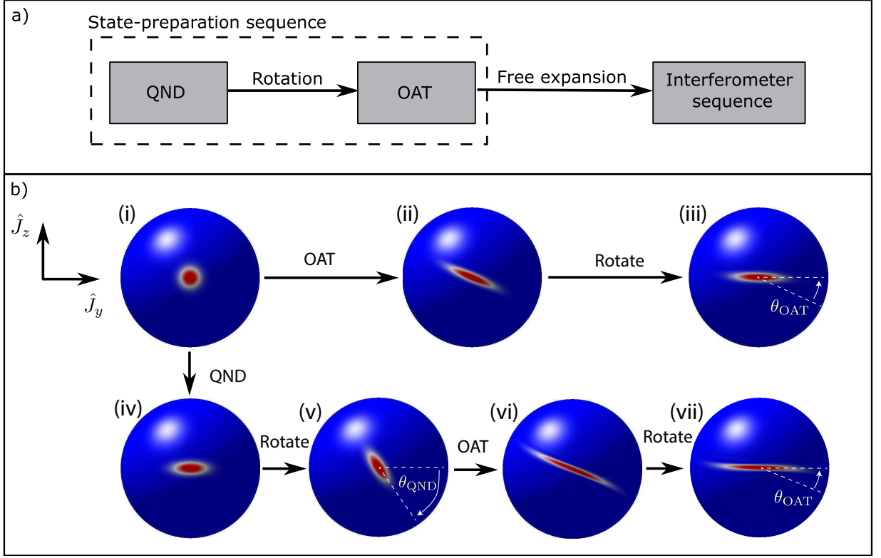
FIG. 1. a) Hybrid method schematic. The model is a modification to the current OAT state-preparation sequence. The output state from the hybrid model is used as the initial state for the interferometer sequence. b) Bloch sphere representation of OAT (top row) and the proposed hybrid method (bottom row) for an initial CSS. In OAT, the initial CSS (i) undergoes nonlinear shearing creating a state with reduced variance in some direction (ii). This state is then rotated about the J_x axis by an amount \theta_{\text{OAT}} in order to create a state with reduced variance in the J_z axis (iii). In the hybrid method, the initial state first undergoes QND squeezing, creating a state with reduced variance in the J_z axis (iv). This state is then rotated about the J_x axis by an amount \theta_{\text{QND}} (v), such that it undergoes more rapid shearing under OAT dynamics (vi). This state is then rotated by amount \theta_{\text{OAT}} to reduce the variance in the J_z direction. When the degree of OAT or QND interaction is limited, the hybrid scheme can produce better spin squeezing than either OAT or QND used in isolation.
