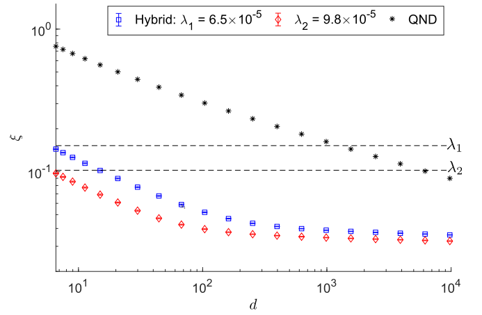
FIG. 7. Squeezing parameter scaling against resonant optical depth of the BEC for only QND (black), and the optimised hybrid method for a OAT interaction strength of \lambda_1 (blue) and \lambda_2 (red). Optical depths of d > 387 require a cavity. The dashed lines represent OAT spin-squeezing at \lambda_1 and \lambda_2 respectively. QND at d = 10^4 represents the best spin-squeezing available in experiments. The hybrid method exceeds this limit for d > 10 at both interaction strengths.
