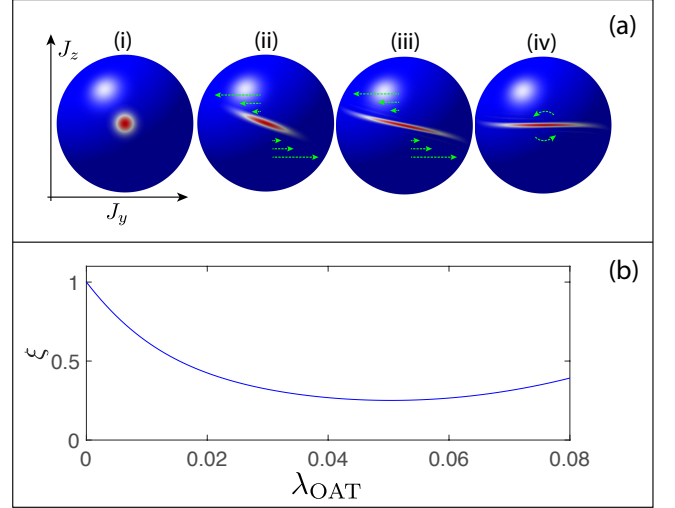
FIG. 4. (a) Evolution of the Wigner quasi-probability distribution for an initial coherent spin state of 100 atoms under OAT dynamics, for (i) \lambda_{\text{OAT}} = 0 , (ii) \lambda_{\text{OAT}} = 0.025 , (iii) \lambda_{\text{OAT}} = 0.05 , (iv) \lambda_{\text{OAT}} = 0.05 , with an additional rotation around the \hat{J}_x axis applied to convert the squeezing into the \hat{J}_z direction. (b): Spin squeezing parameter as a function of \lambda_{\text{OAT}} .
