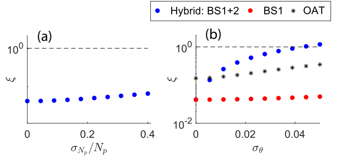
FIG. 8. a) Squeezing parameter scaling against an introduced deviation in photon number (which controls the quantum non-demolition measurement strength) for the hybrid squeezing method. The parameter changes minimally for a deviation up to 30% of the photon number. b) Squeezing parameter scaling against an introduced variance in rotation angle.
