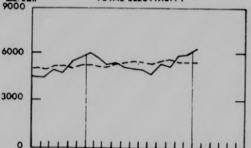
TOTAL ELECTRICITY
