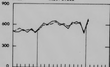
BROWN COAL
