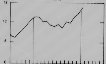
GAS
