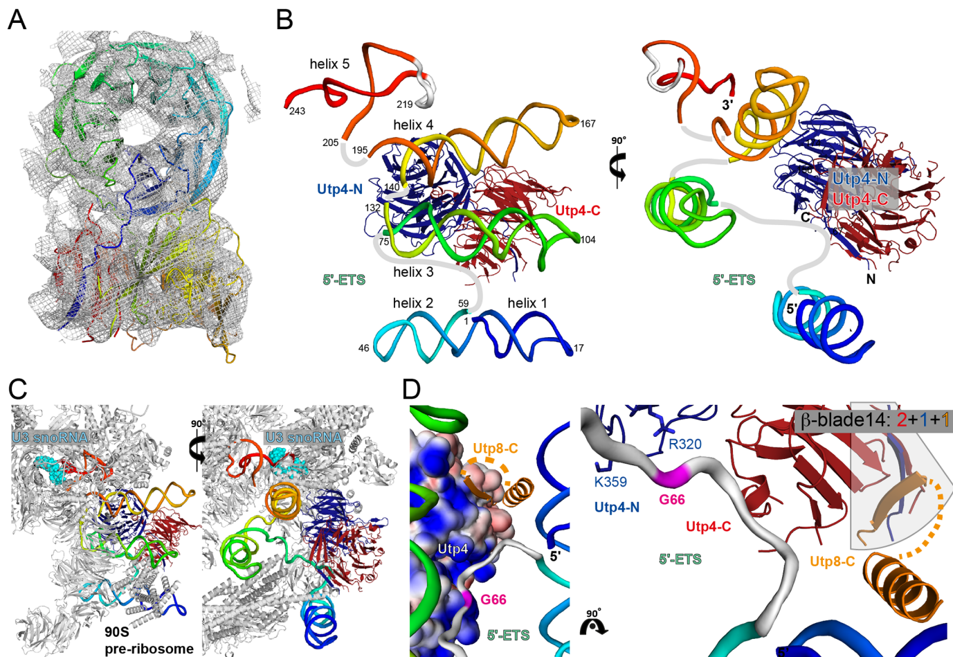
Fig 5. Utp4 in context of the 5'-ETS and 90S pre-ribosome. (A) The crystal structure of Utp4 (rainbow colours) placed into its cryo-EM density (overall 7.3 Å resolution of the particle) in context of the 90S pre-ribosome [9]. The density (grey mesh) is contoured at a 3\sigma level. The Utp4 structure fits in the EM-density as rigid body validating the relative propeller orientation and loop conformations as seen in the crystal structure in the physiological context. (B) Utp4 (blue: propeller 1 (Utp4-N); red: propeller 2 (Utp4-C)) in context of the entire 5'-ETS de novo modeled (rainbow) in the cryo-EM density. RNA helices and nucleotides at special positions are given. The 5'-end is hidden in the continuous stack of RNA helices 1 and 2. Single stranded RNA-parts are indicated by connecting lines (grey). (C) Utp4/5'-ETS in context of a close-up of the UTP-A complex as part of the entire 90S pre-ribosome complex (grey). The region of U3 snoRNA base-pairing at the 3'-end of the 5'-ETS (beyond nucleotide 243) is highlighted in cyan. (D) Utp4/5'-ETS/Utp8 interaction around nucleotide G66 (magenta) identified as major contact point by CRAC analysis. Left panel: Utp4 is indicated by surface potential map ( \pm 5 k_B T/e , blue positive). The C-terminus of Utp8 (Utp8-C, end of predicted \alpha -helix and \beta -strand, no sequence modeled) are given in orange. The \alpha -helix is de novo placed as ideal helix in the cryo-EM density, whereas the \beta -strand is taken from the artificial strand 14D of the X-ray structure (connection given as dashed lines is unclear). Right panel: Model for the Utp8-C interaction with Utp4. The Velcro-closed '2+1+1' blade 14 is completed in trans by Utp8 and G66 binds to the positive patch (indicated by R 344 and K 383 ) in the Utp4-N/Utp4-C interface.
