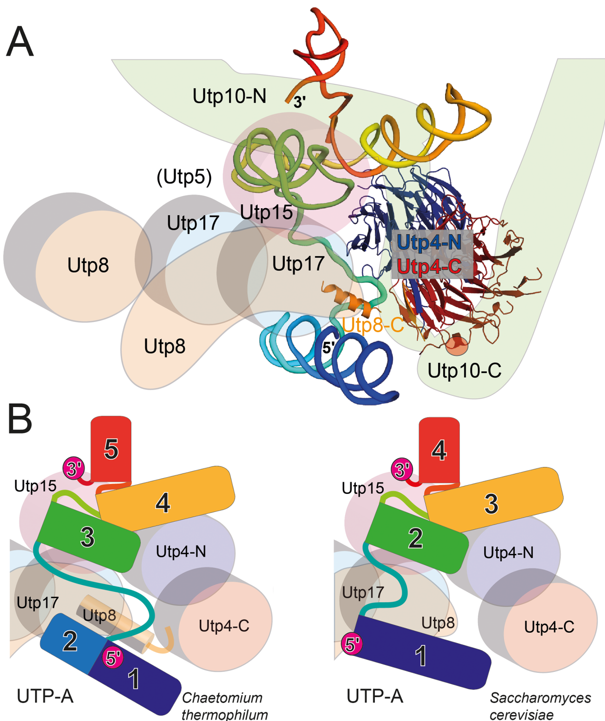
Fig 6. The UTP-A complex from Chaetomium thermophilum . (A) Scheme showing the spatial assembly of the fungal UTP-A complex including the Utp4 X-ray structure and the EM-modeled 5'-ETS. The propellers of remaining UTP-A proteins (Utp8, Utp15, and 2× Utp17) are placed according previous biochemical and EM-studies. The \alpha -solenoidal parts (including whole Utp5) are not included. The entire Utp10 molecule turning around Utp4 is interpreted as also the very C-terminus (atomic model) of Utp8 next to the Velcro-closure of Utp4. The position of the disease-modified arginine in human Utp4 in the interface to Utp10 is highlighted within a red sphere. (B) Comparison of the UTP-A complexes from Chaetomium thermophilum (left panel; [9]) and Saccharomyces cerevisiae (right panel; [27, 28]). While the overall architecture is conserved, the 5'-end of the RNA shows a different arrangement. In addition, the Utp8-Utp4 contact is not visible in the yeast structures.
