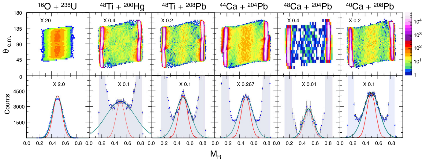
Fig. 1. Measured mass-angle distributions for each reaction (upper panels). The factor multiplies the maximum counts of the logarithmic colour scale (right). In the projected mass ratio spectra (lower panels) the scale factor multiplies the counts scale on the left. The difference between the scale factors is due to the various statistics obtained with each system. Gaussian fits to the region around M_R = 0.5 are shown (turquoise lines), whose standard deviations \sigma are given in Table 1. Gaussian functions with \sigma_{MR} = 0.07 (thin red lines) are shown for reference. (For interpretation of the references to colour in this figure legend, the reader is referred to the web version of this Letter.)
