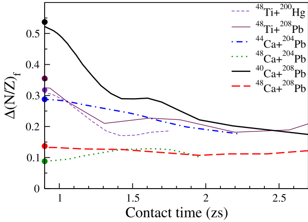
Fig. 3. Final N/Z asymmetry of the fragments (lines) as a function of contact time of the fragments in zeptoseconds ( 1 \text{ zs} = 10^{-21} \text{ s} ), defined as the time during which the neck density exceeds half the saturation density \rho_0/2 = 0.08 \text{ fm}^{-3} . The initial values \Delta(N/Z)_i are shown by full circles.
