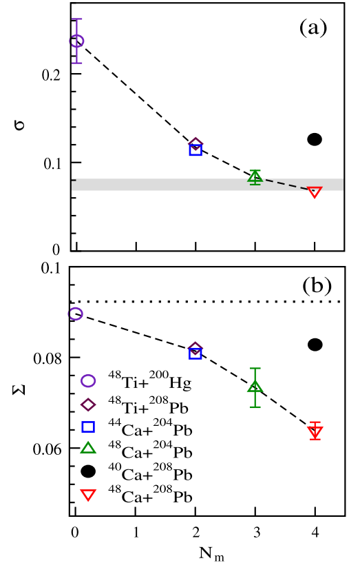
Fig. 2. (a) Standard deviations \sigma_{MR} of the Gaussian fits of the fission-like fragment mass distributions as a function of the number of magic numbers in the entrance channel N_m . The horizontal band shows the upper limit of \sigma_{MR} for pure fusion–fission (i.e., without QF). (b) Standard deviation \Sigma_{MR} in the 0.34 \leq M_R \leq 0.66 range. The dotted line corresponds to a flat distribution. When not shown, the statistical uncertainties are smaller than the size of the points. The dashed lines guide the eye.
