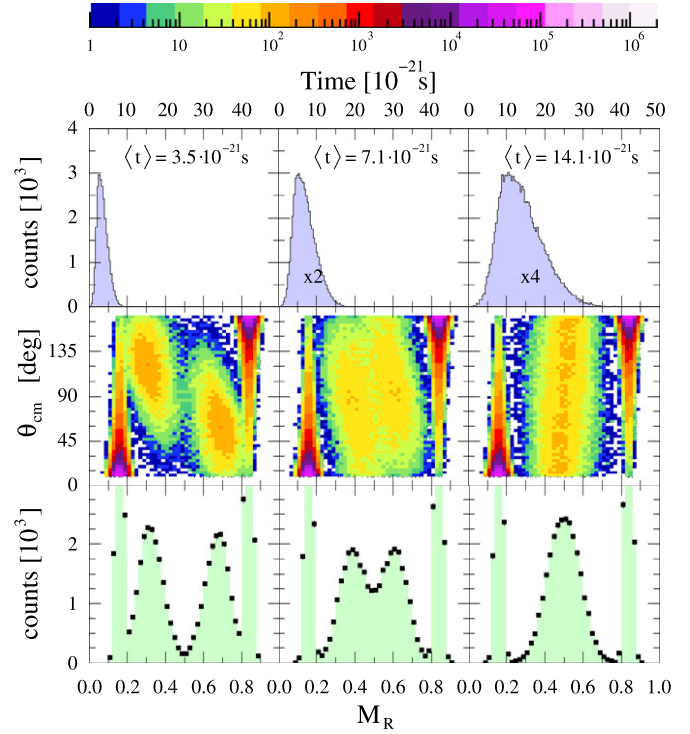
Fig. 4. Simulated mass-angle distributions (middle panels) for ^{40}\text{Ca} + ^{208}\text{Pb} following [9], for the quasi-fission time distributions shown in the upper panels. The average time \langle t \rangle of these distributions is indicated. The projections on the mass ratio axis are shown in the lower panels.
