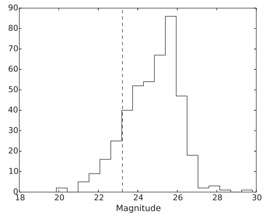
Figure 2. The luminosity function for all spatially unresolved [O III] emitters identified in the combined left and right images of the PN.S for NGC 6946. The dashed line shows the expected bright luminosity cut-off for PNe. Objects brighter than the cut-off are probably bright H II regions.
