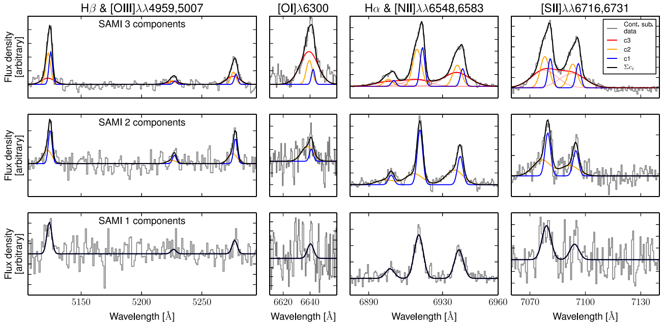
Figure 3. Examples of our spectral decomposition using the SAMI data. First, second and third rows are examples of selected spaxels requiring three-component, two-component and one-component fits to describe the spectral profiles, respectively. Each panel is a zoom-in of the spectral ranges comprising key diagnostic emission lines. Continuum subtracted spectra are shown in grey. Best-fitting c3 , c2 , and c1 are shown in red, orange, and blue, respectively. The best-fitting emission line models, i.e. \sum c_i , are shown in black. To avoid confusion in cases where the lines are broad and blended, we also show individual line transitions of c3 as transparent red lines. Details of our spectral analysis technique are described in Section 4.
