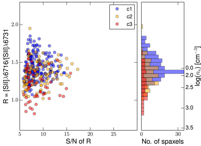
Figure 10. Left: [\text{SII}] \lambda 6716 to [\text{SII}] \lambda 6731 line ratios versus S/Ns of the line ratios as measured from the SAMI data. A minimum flux S/N of eight is applied on both lines. Measurements from different components are colour-coded as indicated in the legend. Right: histogram of their data in the left-hand panel. We show the inferred electron densities from the [\text{SII}] ratios on the y-axis on the right-hand-side. Although the density measurements are low in S/N, it is evident that c3 has systematically low electron densities than c1 .
