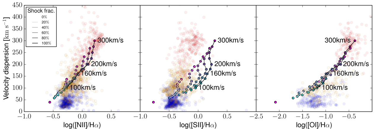
Figure 14. Velocity dispersion mixing sequence as predicted by our photoionization and shock models. The line segments connect model grids of certain shock fractions with changing shock velocities. Grey-scales of the segments correspond to different shock fractions as indicated in the legend. The shock velocity grids have increments of 20 \text{ km s}^{-1} between 100 and 200 \text{ km s}^{-1} , and increments of 25 \text{ km s}^{-1} between 200 and 300 \text{ km s}^{-1} . The 0 per cent shock fraction points (lower-left corners) are models of pure photoionization of \text{H II} regions of \log(q) = 7.5 \text{ cm s}^{-1} , and 12 + \log(\text{O}/\text{H}) = 9.14 (Dopita et al. 2013). Blue, orange, and red transparent data points are SAMI measurements of the different kinematic components shown in Fig. 8. Details of the models are provided in Section 6.2.1.
