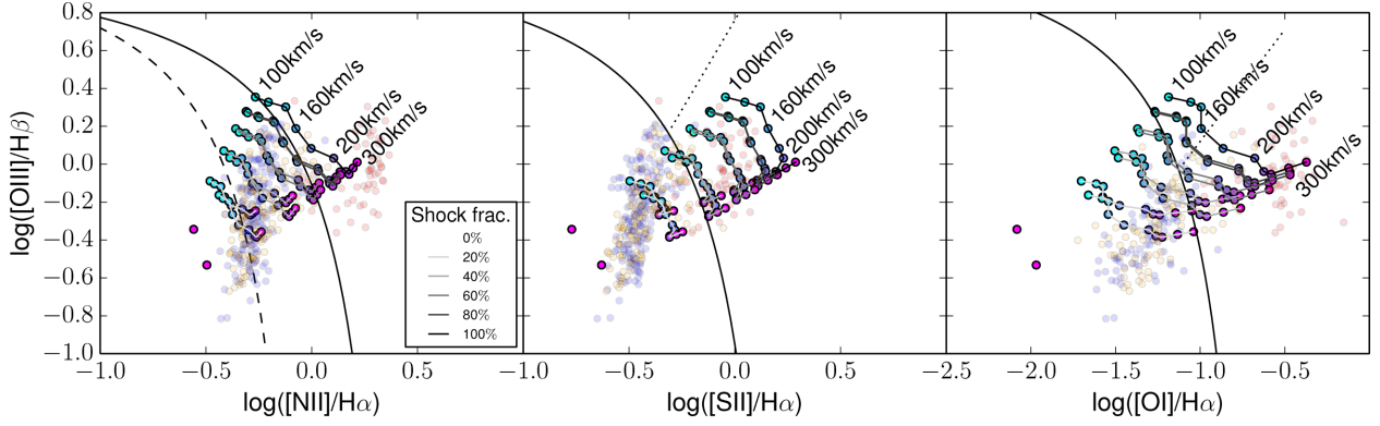
Figure 13. Shock and photoionization mixing sequences predicted by our models. The line segments connect model grids of certain shock fractions with changing shock velocities. Different grey-scales of the segments correspond to different shock fractions as indicated in the legend. The shock velocity grids have increments of 20 \text{ km s}^{-1} between 100 and 200 \text{ km s}^{-1} , and increments of 25 \text{ km s}^{-1} between 200 and 300 \text{ km s}^{-1} . The two sets of 0 per cent shock fraction points (lower-left corners) are models of pure photoionization of \text{H II} regions of \log(q) = 7.5 \text{ (cm s}^{-1}\text{)} ; upper data point) and 7.25 \text{ (cm s}^{-1}\text{)} ; lower data point), and 12 + \log(\text{O}/\text{H}) = 9.14 (Dopita et al. 2013). Blue, orange, and red transparent data points are SAMI measurements of the different kinematic components shown in Fig. 8. Details of the models are provided in Section 6.2.1.
