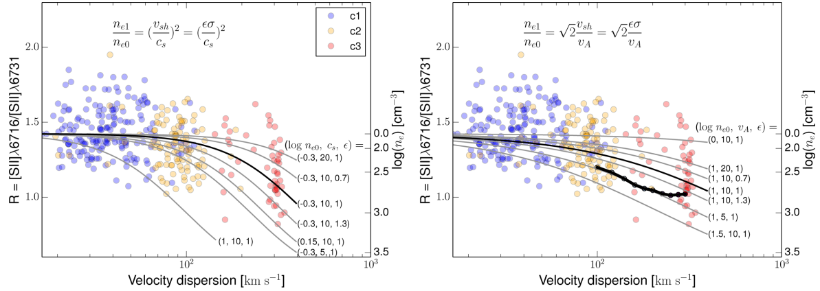
Figure 15. [S II] ratios and electron densities, versus velocity dispersion for the SAMI data shown in Fig. 10. Filled circles of different colours represent different components as shown in the legend. The curves are models of isothermal shocks propagating in ISM without magnetic field (left-hand panel) and with magnetic field (right-hand panel). The models described by equations (4) and (5) are also labelled in the two panels. The models providing the best representation of the data are shown as the black curves. The models with different parameters close to those of the black models are shown in grey. The three parameters adopted in each model are labelled next to each curve. The units are \text{cm}^{-3} for the pre-shock electron density ( n_{e0} ), and \text{km s}^{-1} for the sound speed ( c_s ) and Alfvén velocity ( v_A ). The geometric factor ( \epsilon ) is unit-less. The predictions from the MAPPINGS IV shock models are shown as thick black segments in the right-hand panel. Details are discussed in Section 6.2.1.
