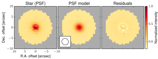
Figure 11. Left: normalized narrow-band image (6400–6500 Å) reconstructed from the data cube of a calibration star. The star was observed simultaneously with the galaxy by SAMI. Middle: 2D Gaussian fit of the narrow-band image. The Gaussian has a FWHM size of 3.2 \text{ arcsec} \times 3.0 \text{ arcsec} and a position angle of -33^\circ , as also indicated by the ellipse in the bottom-left corner. Right: residuals of the model fit.
