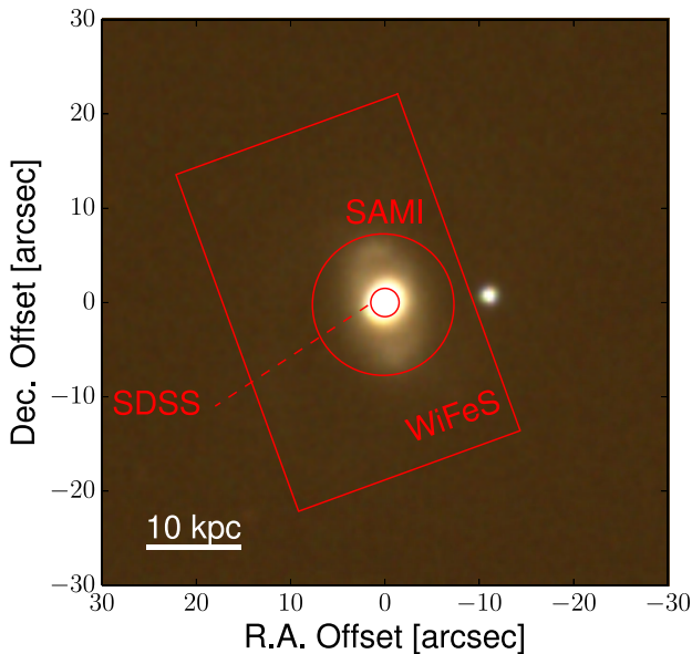
Figure 1. SDSS g, r, i colour composite image overplotted with footprints of SDSS, SAMI and WiFeS. The SDSS fibre has a diameter of 3 arcsec. The SAMI hexabundle has a circular FOV of 15 arcsec in diameter, and the WiFeS image-slicing IFU has an FOV of 25 \text{ arcsec} \times 38 \text{ arcsec} .
