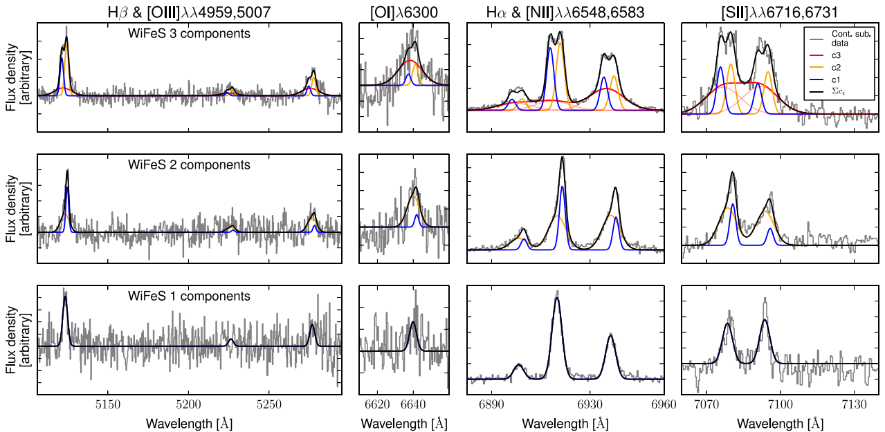
Figure 4. Same as Fig. 3 but for the WiFeS data.
