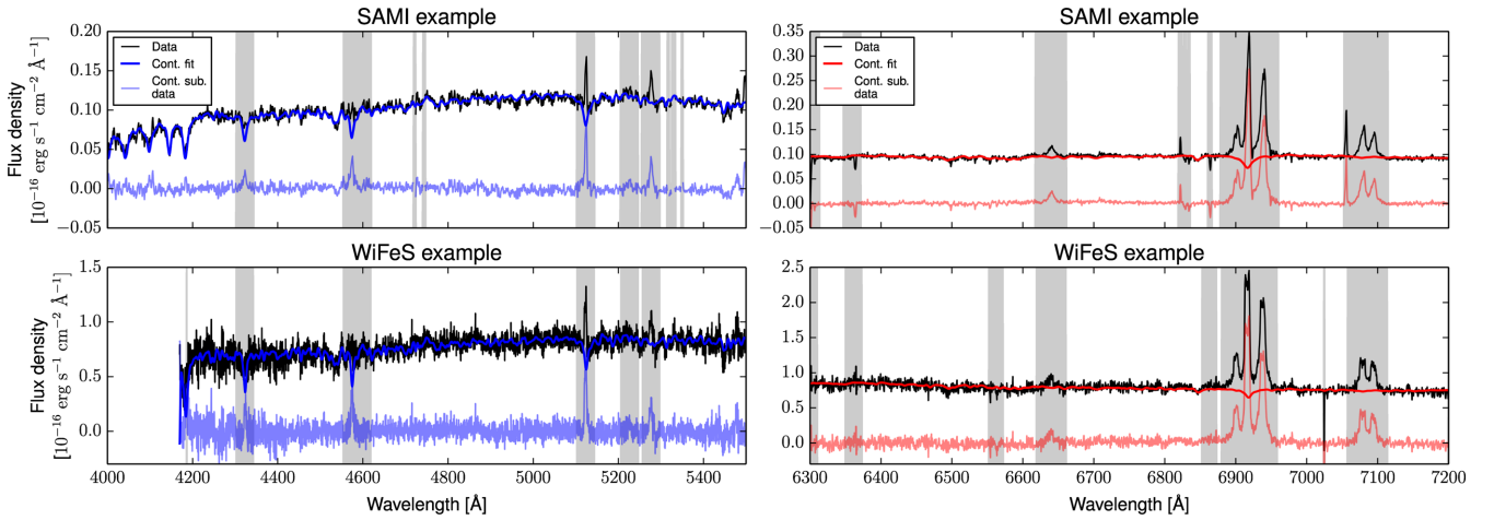
Figure 2. Examples of SSP synthesis fitting using PPXF and stellar models by González Delgado et al. (2005). The upper panels and lower panels show examples of the SAMI and WiFeS data of SDSS J0900, respectively. The same two spaxels are also presented in the upper panels of Figs 3 and 4 to demonstrate spectral decomposition. The blue (left-hand panels) and the red (right-hand panels) spectra are shown separately. Grey bands mark bad channels, channels around sky lines, or strong emission lines that were not included in the continuum fitting. Details are provided in Section 4.
