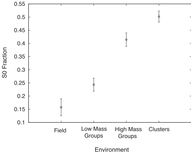
Figure 2. Fraction of galaxies in the field, low [ \log(M_\odot) < 13 ] and high [ 13 < \log(M_\odot) < 15 ] mass groups, and clusters which are classed as S0. The error bars denote the 95 percent bimodal confidence intervals. As expected from previous results, the number of S0 galaxies steadily increases with the increasing density.
