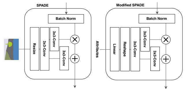
Figure 2: Original SPADE block (left) and our modified version (right).
