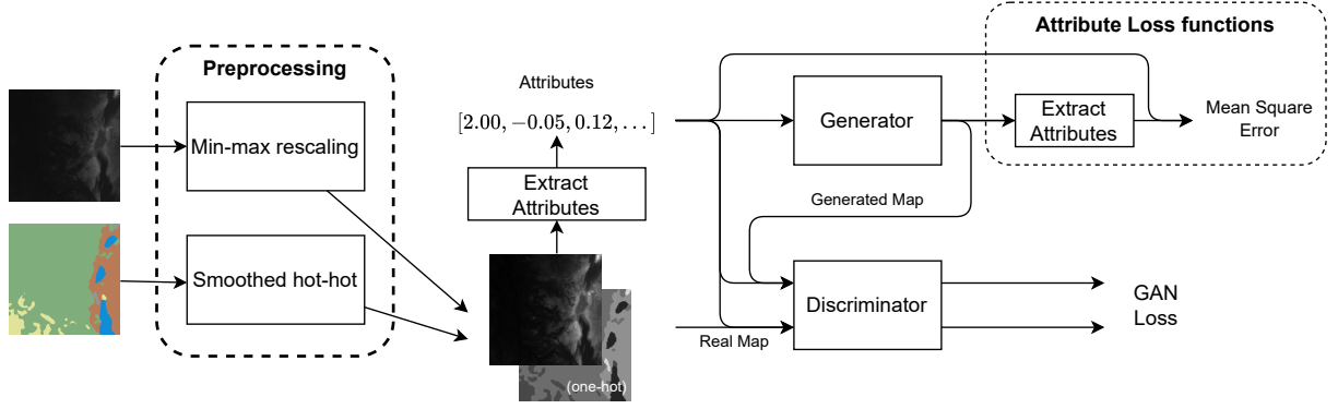
Figure 1: Overall workflow: preprocess the dataset, extract attributes, then train the model with the attribute loss functions.
