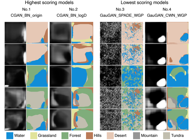
Figure 4: Samples generated by the two models with the highest NRDS (left), and two lowest (right). The grayscale images are height maps and the coloured images are segmentation maps. Each row contains samples with the same attributes.
