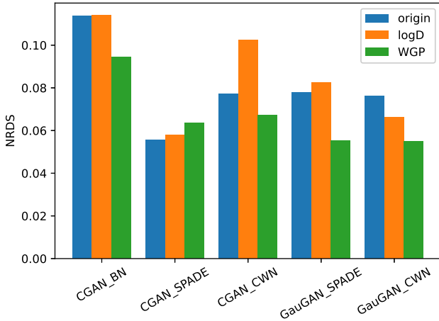
Figure 3: NRDS for each combination of models, normalisation methods, and loss functions.
