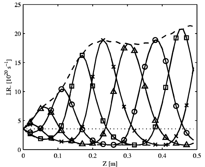
FIG. 10. Instantaneous ionization rate model for electric fields determined by the AntennaII code in Fig. 9(b). The instantaneous rate curves each correspond to a quarter rf period later in time. The dotted line corresponds to the ionization rate from a 3 eV Maxwellian distribution.
