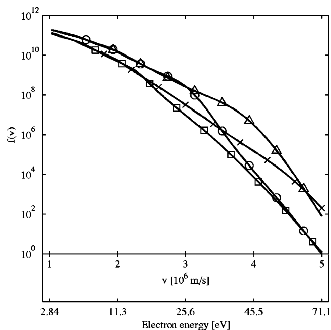
FIG. 12. Time dependence of wave-excited electron distribution function at z = 34 cm. Each line connecting squares, crosses, triangles, or circles represents the distribution function a quarter of an rf cycle later which is 18.4 ns for the 13.56 MHz source.
