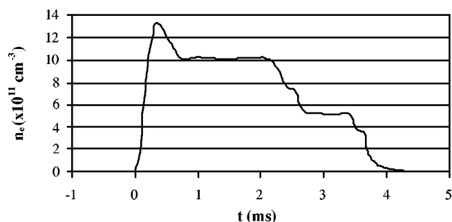
FIG. 3. Langmuir probe density trace versus time at z = 20 \text{ cm} , r = 3 \text{ cm} .
