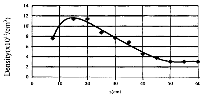
FIG. 4. Measured axial density profile at r = 3 \text{ cm} .
