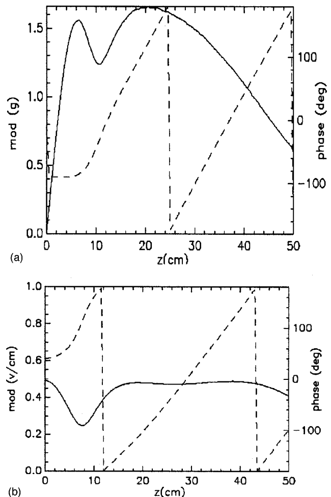
FIG. 9. AntennaII modeling of measured B_z [mod(g)] (a) at r=4 cm and corresponding wave E_z [mod(v/cm)] (b) at r=6.3 cm. The solid line represents amplitude and the dashed line represents phase.
