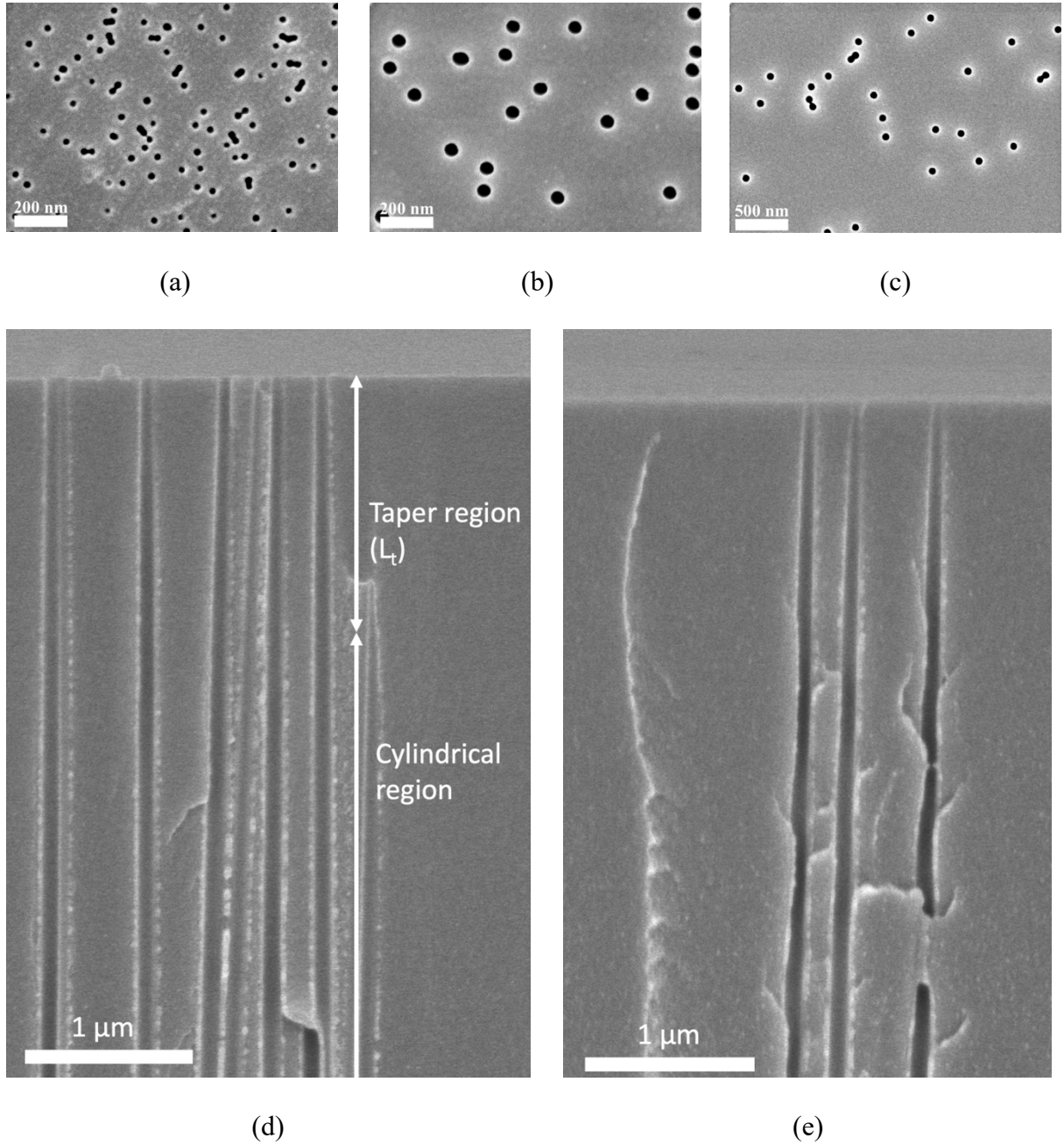
Figure 8: SEM images of nanopores fabricated in PC membranes irradiated with different fluences and etched for different times in 5M NaOH at 60°C (a) plan-view with a fluence of 1 \times 10^{10} ions \text{cm}^{-2} and etched for 90 s. (b) plan-view with a fluence of 1 \times 10^9 ions \text{cm}^{-2} and etched for 180 s. (c) plan-view with a fluence of 3 \times 10^8 ions \text{cm}^{-2} and etched for 270 s. Cross-section SEM towards top surface (d) and bottom surface (e) of the membrane irradiated with a fluence of 3 \times 10^8 and etched for 210 s. Taper region and cylindrical region are indicated in (d) .
