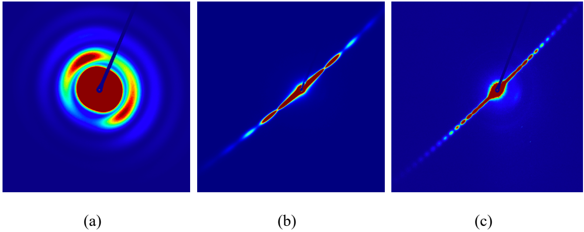
Figure 2: Detector images (2D scattering patterns) of PC membranes with parallel oriented nanopores: pore axis aligned to X-ray beam (a), and samples tilted by an angle of 10^\circ with respect to the X-ray beam for a membrane irradiated with a fluence of 1 \times 10^9 ions \text{cm}^{-2} and etched for 60 s (b) and a membrane irradiated with a fluence of 1 \times 10^8 ions \text{cm}^{-2} and etched for 270 s (c). The central part of the detector is protected against the primary beam by a beam stop.
