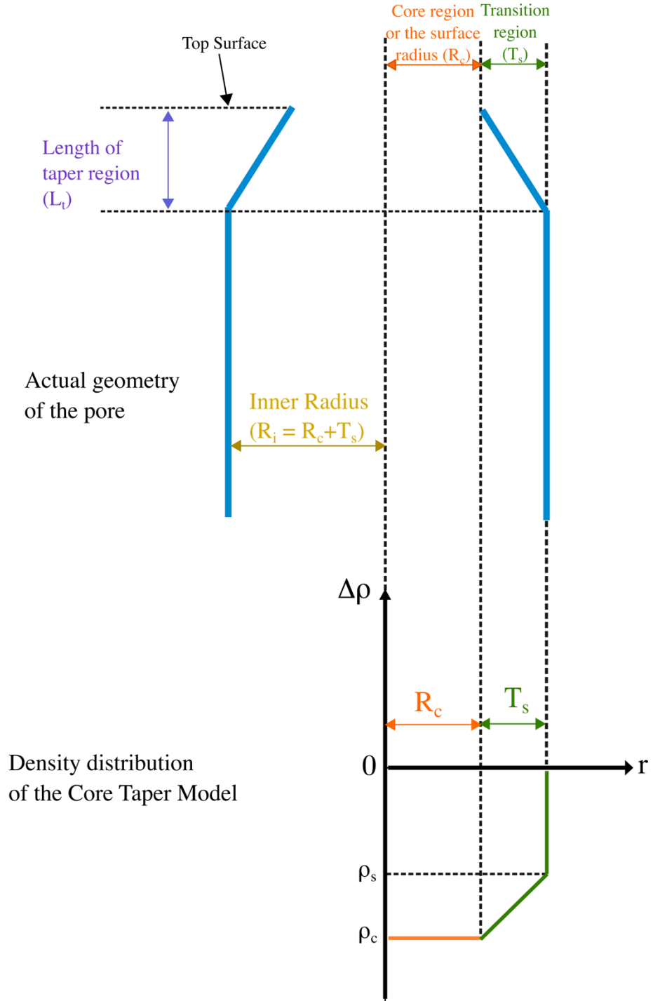
Figure 3: Graphical representation showing the relation between the radial electron density profile for the Core Taper Model (bottom) and the actual geometry of the pore (top). Only the top half of the pore is shown for easy visualisation.
