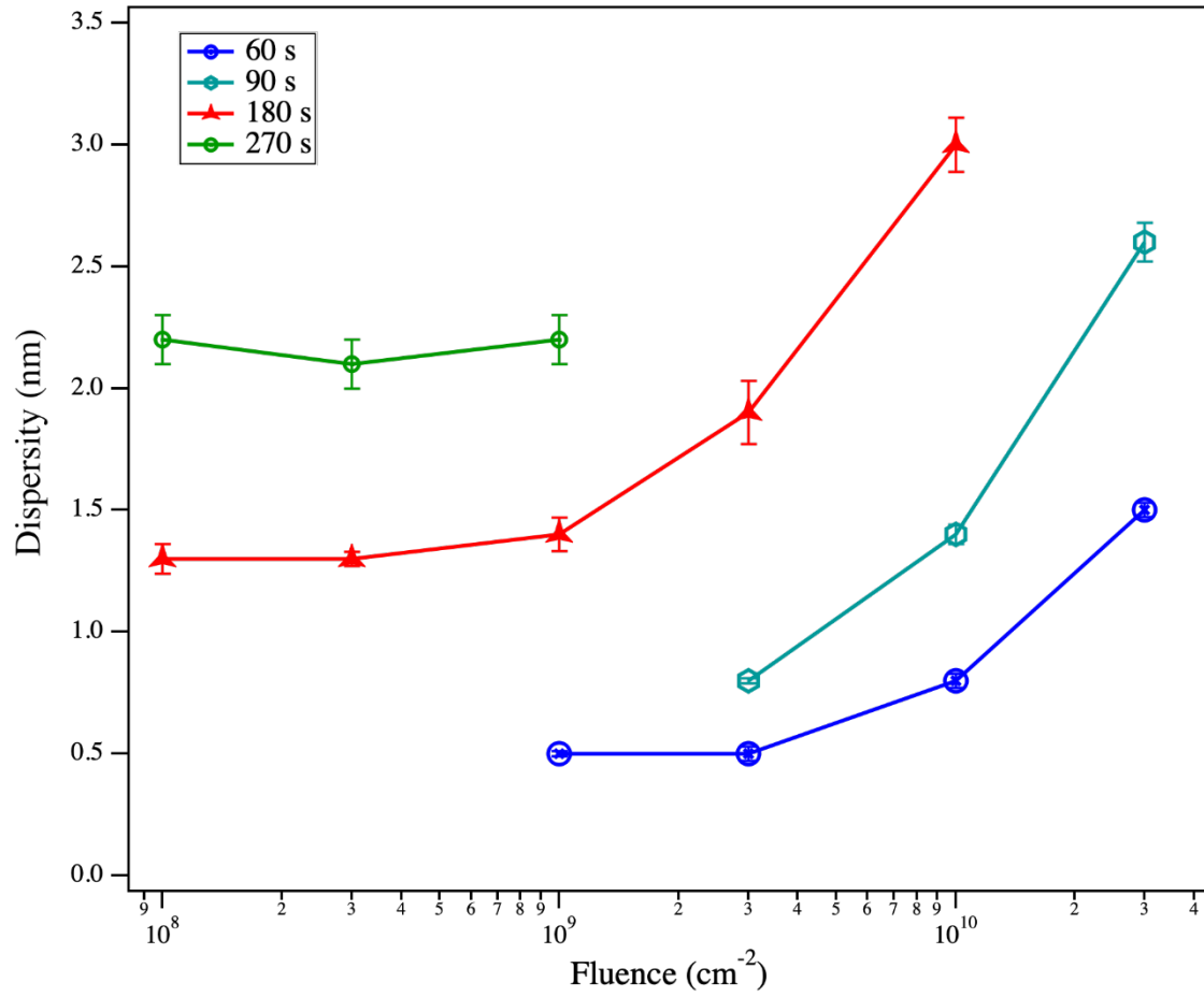
Figure 10: Size dispersity as a function of fluence for different etching times (nanopore size). The dispersity increases for fluences larger than 1 \times 10^9 ions/cm 2 .
