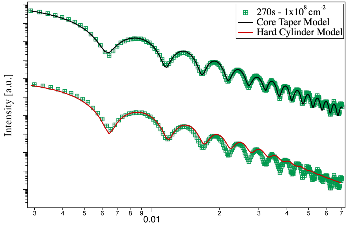
Figure 5: Integrated SAXS scattering intensities for a PC membrane irradiated with 1 \times 10^8 ions \text{cm}^{-2} and etched for 270 s. The solid lines represent the numerical fit using the Core Taper Model (black) and the Hard Cylinder Model (red). The scattering oscillations at higher q values fit significantly better using the Core Taper Model compared to the Hard Cylinder Model.
