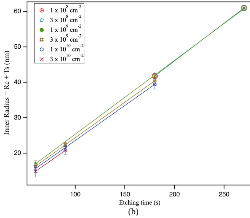
Figure 11: Nanopore radii as a function of etching time for different fluences, The results are deduced from fits to SAXS data using the Core Taper Model: (a) surface radius and (b) inner radius of nanopores . Linear fits(solid lines) to the data yields radial etch rates.
