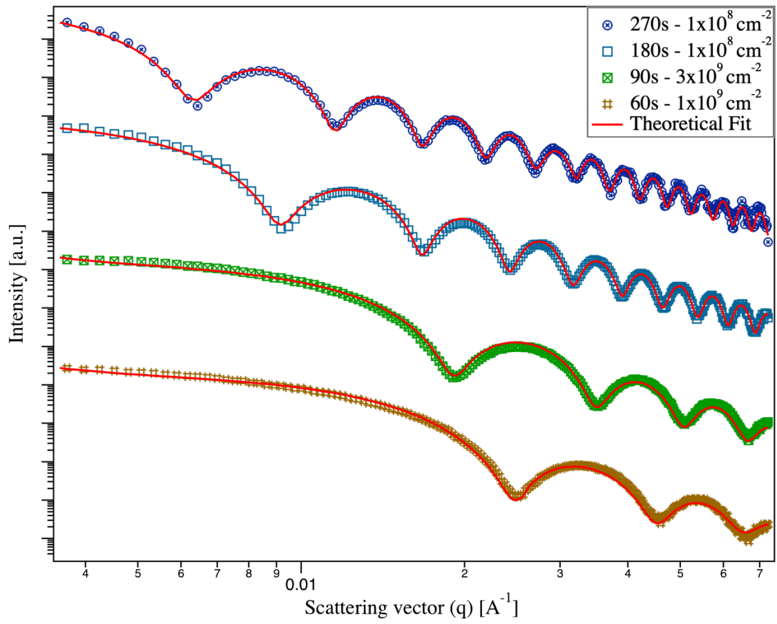
Figure 6: Integrated SAXS scattering intensities for samples etched for different times. The solid red lines represent the numerical fits obtained using the Core Taper Model.
