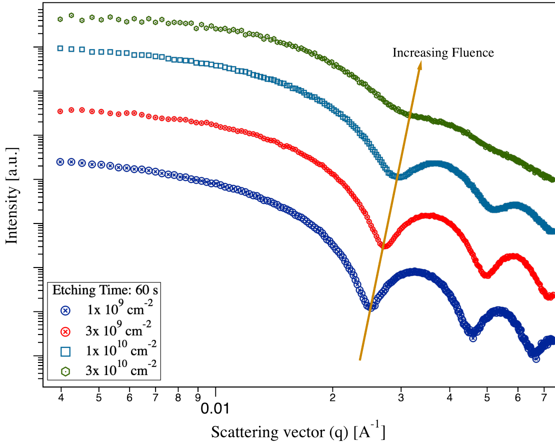
Figure 4: Integrated SAXS scattering intensities for PC samples irradiated with different fluences and etched for 60 s (5 M NaOH at 60° C). The shift in the oscillations of the scattering intensities is due to a decrease in pore radius with increasing fluence. The smearing out of the oscillations indicates increasing dispersity for higher fluences. The patterns are stacked for better visibility.
