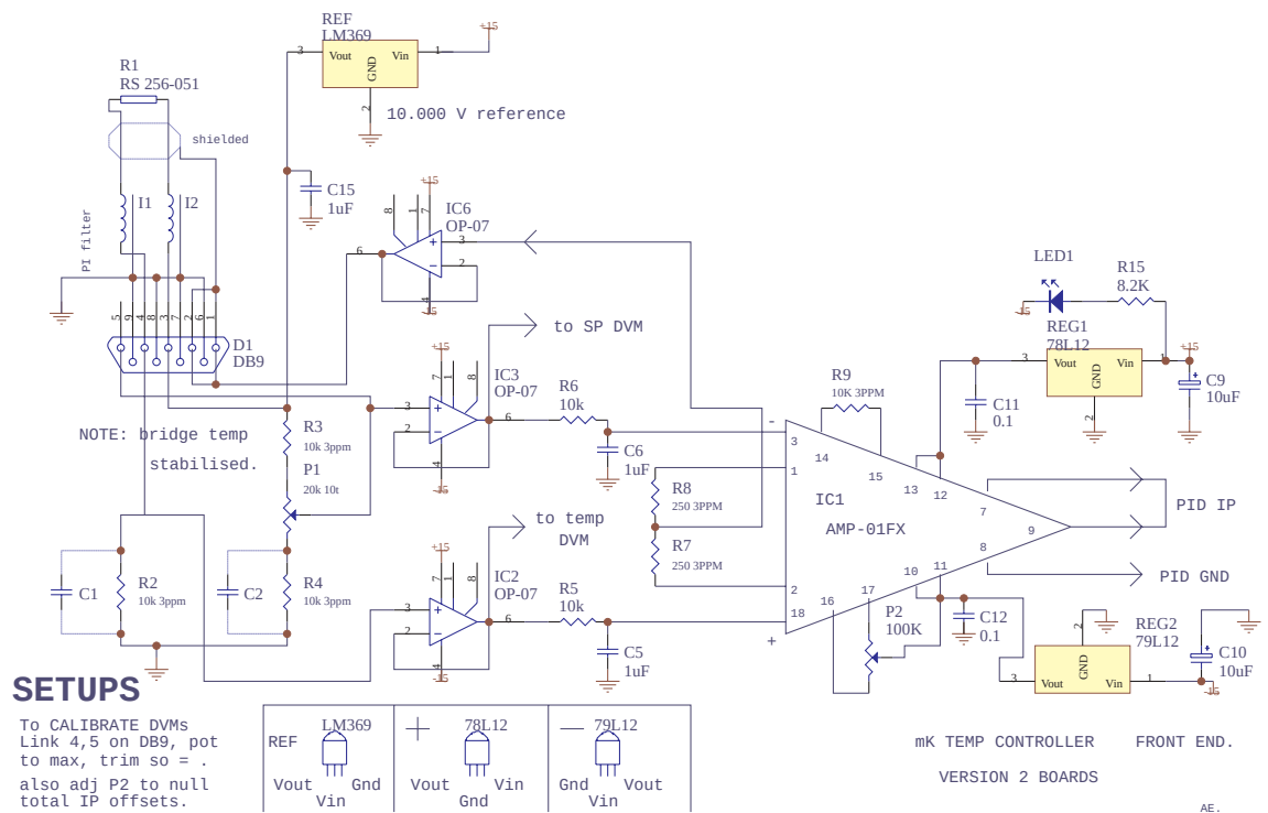
Figure D.1: Front end interface of milli-Kelvin temperature controller.
