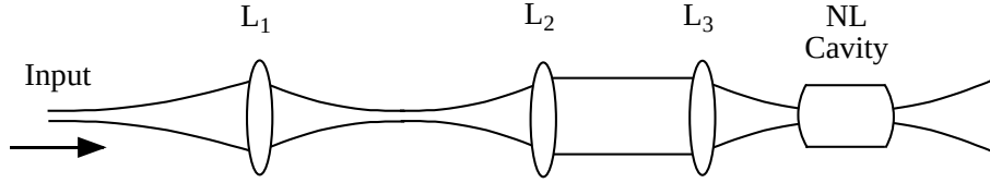
Figure 3.1: Precise mode matching of a Gaussian beam via telescopic lens arrangement. L_1 is used to achieve the desired beam waist. The L_2 and L_3 combination is used to translate the desired beam waist to the location of the nonlinear optical cavity.
