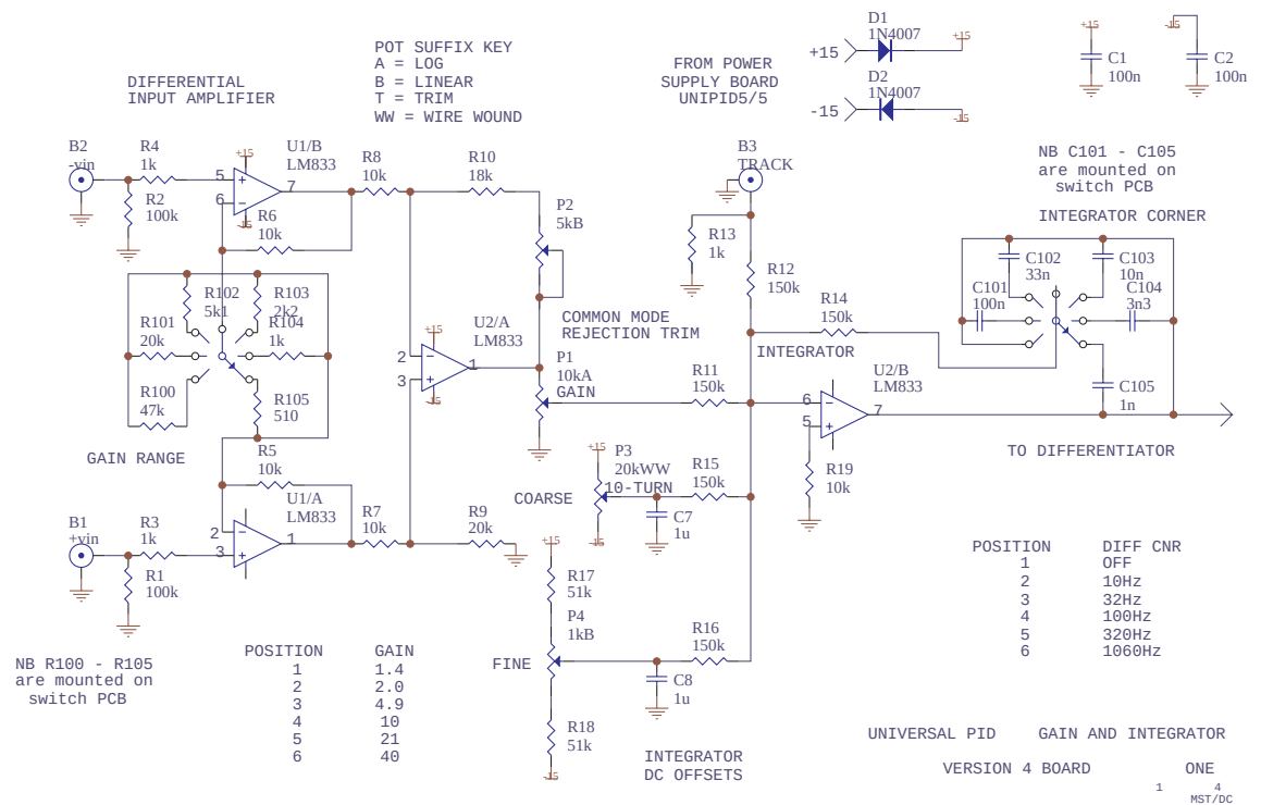
Figure C.1: Gain and integration stages of UniPID 5.0.
