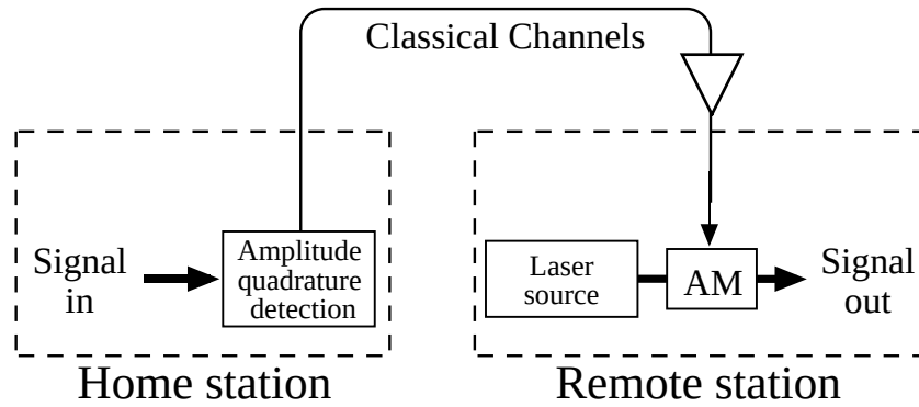
Figure 11.1: Simple transmission scheme.
