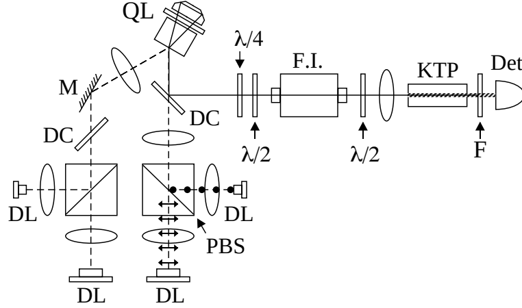
Figure F.2: Schematic of the Q-switched second harmonic generator. PBS: Polarizing beam splitter; DC: Dichroic beam splitter; DL: Diode laser array; QL: Q-switched laser; M: Mirror; \lambda/2 , \lambda/4 : Half and quarter wave plates, respectively; FI: Faraday isolator and F: IR Filter.
