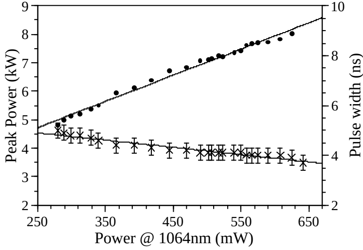
Figure F.3: Q-switched output pulse frequency (dots) and pulse width (crosses) vs average fundamental power.
