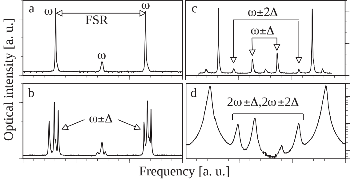
Figure 6.3: Optical spectrum analyser outputs of the intra-cavity NDOPO modes. Optical intensity is plotted against frequency (detuning of the OSA) in arbitrary units. (a) shows a single FSR scan of the OSA with only the 1064 nm input, the small peak in the middle of the FSR is due to imperfect alignment of the cavity. (b) the onset of intra-cavity NDOPO at P_1 = 14 mW gives rise to an additional pairs of fundamental modes at frequency \omega \pm \Delta . (c) At even higher fundamental pump power, P_1 = 49 mW, two pairs of nondegenerate fundamental modes emerged. Finally using another OSA for the second harmonic modes (d) shows that at P_1 = 155 mW, the intra-cavity NDOPO is strong enough to generate their own optical harmonic. The intensity scale is logarithmic for (d).
