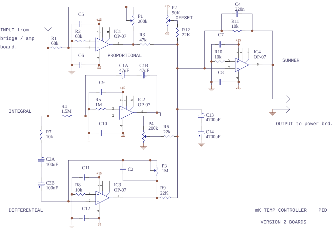
Figure D.2: PID circuit of milli-Kelvin temperature controller.
