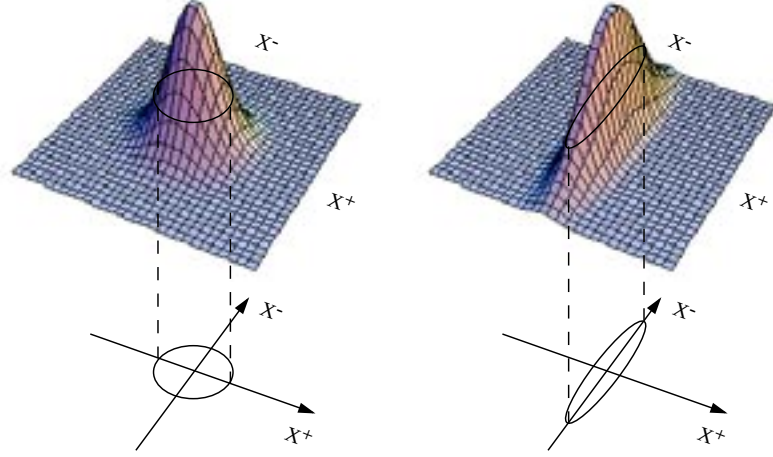
Figure 2.5: Correspondence between Wigner representation and the ball-on-stick representation
