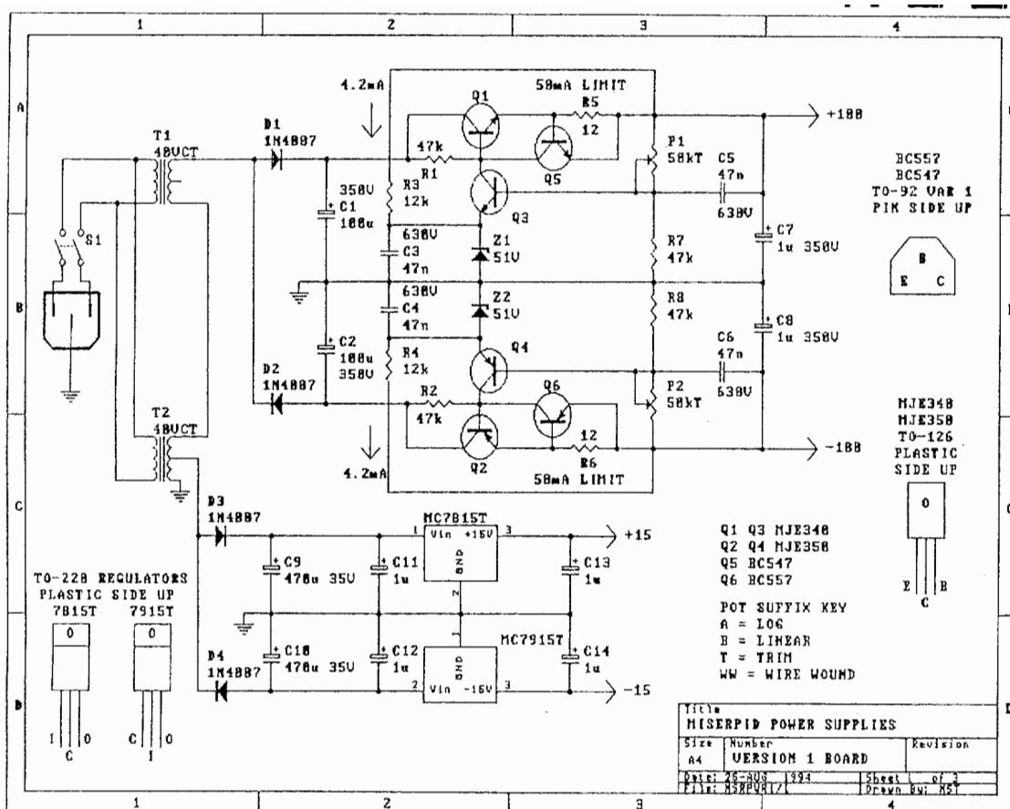
Figure E.4: Laser controller power supply.
