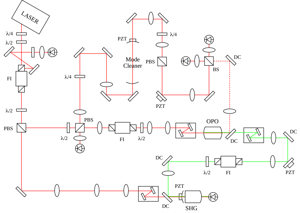
Figure 8.1: The experimental setup of the squeezed vacuum generator. \lambda/2 , \lambda/4 : half, and quarter wave plates; FI: Faraday isolator; BS: 50/50 beam splitter; PBS: Polarizing beam splitter; DC: Dichroic; PZT: Piezo-electric actuator.
