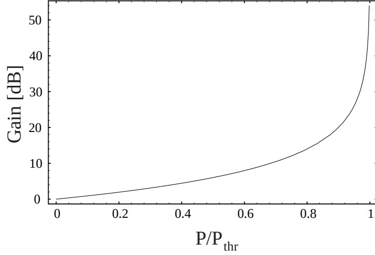
Figure 8.2: Calculated classical gain of the OPO operating as an amplifier. The gain is calculated by considering the ratio of transmitted powers with OPO pump power on and off, P_{\text{inc}} = P and P_{\text{inc}} = 0 .
