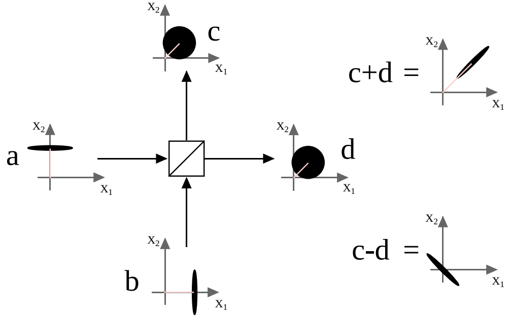
Figure 11.5: EPR entanglement.
