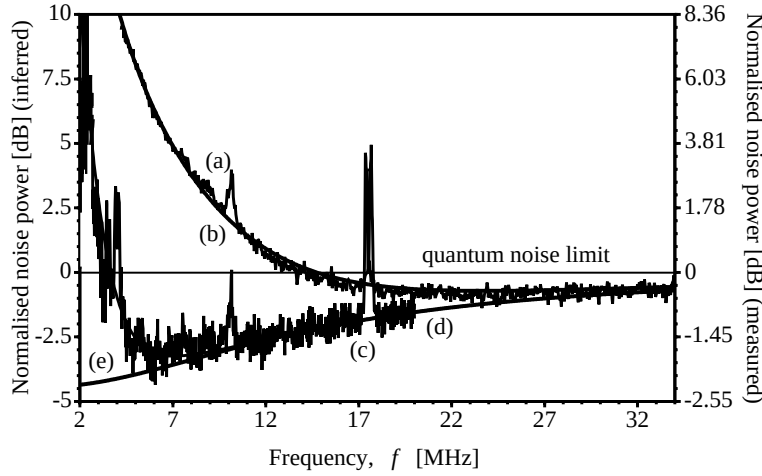
Figure 5.4: Theoretical and experimental spectra of the SHG. Traces (a) and (c) are the spectra obtained for the experiment run without and with the mode cleaner, respectively, after correction for electronic noise. The maximum squeezing in each case are 0.47 dB (0.75 dB inferred) at 23 MHz for trace (a) and 1.7 dB (3.0 dB inferred) at 7.5 MHz for trace (c). The small noise peak at 10 MHz on both traces is the residual noise from the locking system. Traces (b) and (d) are the theoretical plots corresponding to the experimental traces. Trace (e) is the theoretical prediction for the second harmonic squeezing with a coherent pump (quantum noise limited at all frequencies).
