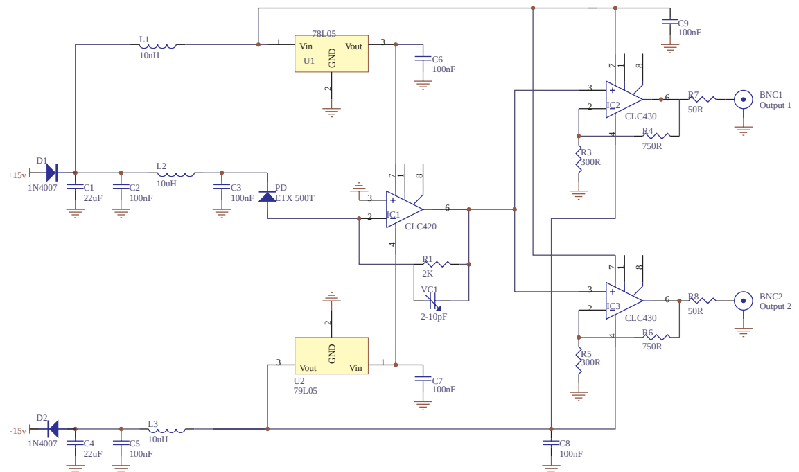
Figure B.1: Circuit diagram of 1064 nm photodetector. The photodiode used is ETX-500 from Epitaxx. RF operational amplifiers use are Comlinear CLC-420 and CLC-430.
