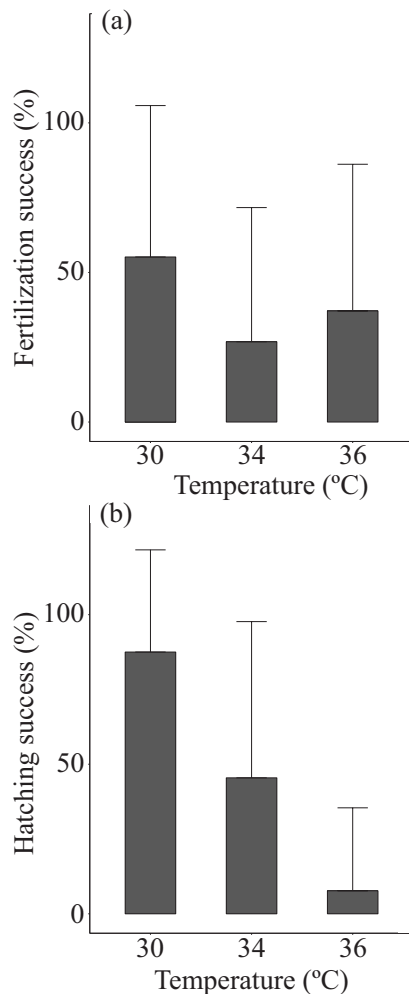
Figure 2. The effect of temperature on fertilization (A) and hatching success (B).
