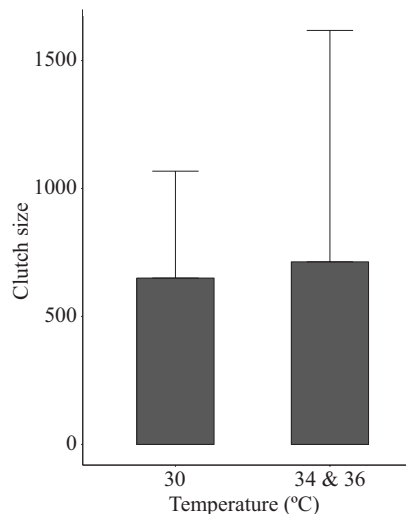
Figure 7. The effect of temperature on clutch size.
