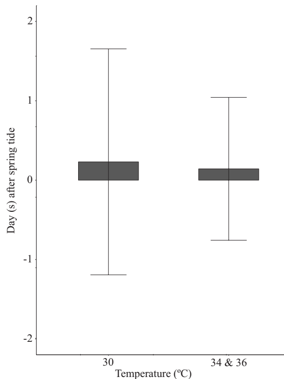
Figure 6. The effect of temperature on the mismatch of larval release day.
