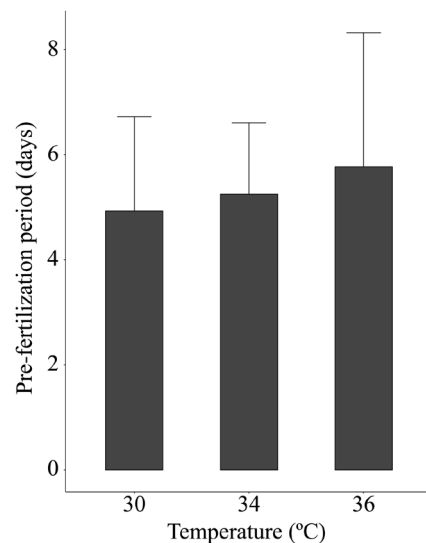
Figure 4. The effect of temperature on the pre-fertilization period.
