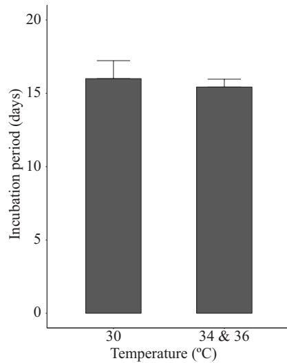
Figure 5. The effect of temperature on the incubation period.
