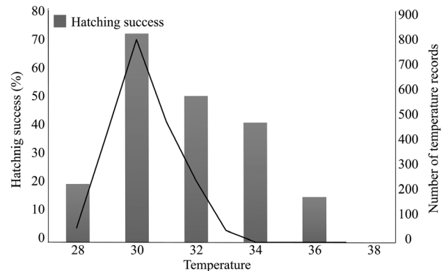
Figure 3. Hatching success from the combined dataset (i.e. our data and data from Clark & Backwell (2016)). Plot with data from Clark & Backwell (2016) showing the distribution of in total 2070 temperature readings in natural burrows during October–December 2012.
