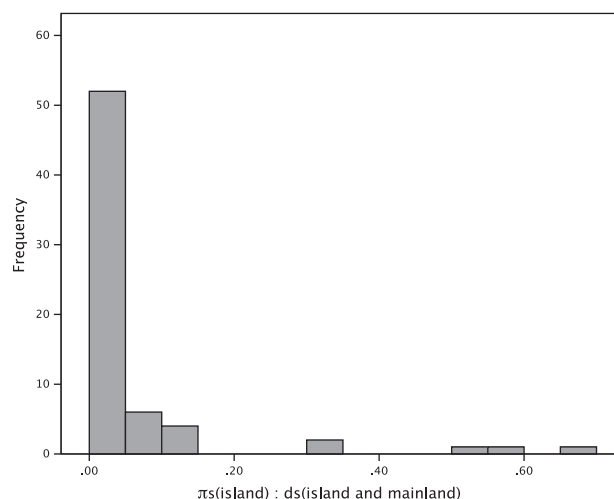
FIG. 3. —Frequency distribution of the ratio of island \pi_S : island and mainland d_S .
