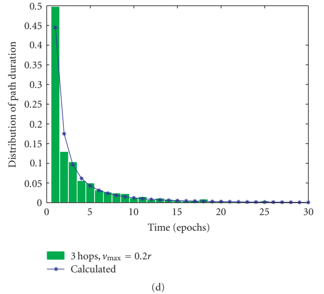
FIGURE 8: Comparison of metric calculations and simulated results for path residual time and path duration. Each MN moves at a randomly chosen velocity during each epoch, which has uniformly distributed speed in the range [0, v_{\max}] and uniformly distributed direction in the range [0, 2\pi) . (a) Comparison of calculated and experimental average path residual time values for bounded and unbounded simulation areas and BFS algorithm. Calculated values are from (40). (b) Comparison of calculated and experimental average path duration values for bounded and unbounded simulation areas and BFS algorithm. Calculated values are from (42). (c) Comparison of calculated and experimental distributions of the path residual time for an unbounded simulation area. Calculated values are from (39). (d) Comparison of calculated and experimental distributions of the path duration for an unbounded simulation area. Calculated values are from (39).
