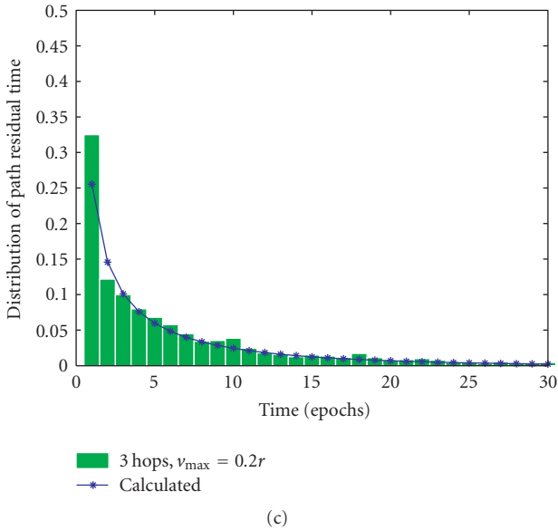
FIGURE 8: Comparison of metric calculations and simulated results for path residual time and path duration. Each MN moves at a randomly chosen velocity during each epoch, which has uniformly distributed speed in the range [0, v_{\max}] and uniformly distributed direction in the range [0, 2\pi) . (a) Comparison of calculated and experimental average path residual time values for bounded and unbounded simulation areas and BFS algorithm. Calculated values are from (40). (b) Comparison of calculated and experimental average path duration values for bounded and unbounded simulation areas and BFS algorithm. Calculated values are from (42). (c) Comparison of calculated and experimental distributions of the path residual time for an unbounded simulation area. Calculated values are from (39). (d) Comparison of calculated and experimental distributions of the path duration for an unbounded simulation area. Calculated values are from (39).
