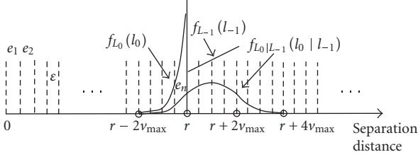
FIGURE 4: Depiction of PDFs of node separation, with respect to separation distance state space, at epochs -1 and 0 , taking into account moves that do and do not result in a link being established. Nodes are assumed to be uniformly distributed.
