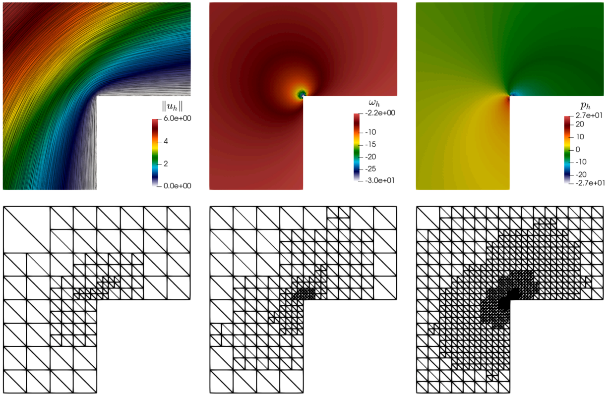
Fig. 3. Sample of approximate solutions for the convergence test on an L-shaped domain (top rows), and coarse meshes produced after three, six, and nine steps of the adaptive refinement algorithm guided by the a posteriori error estimator.
