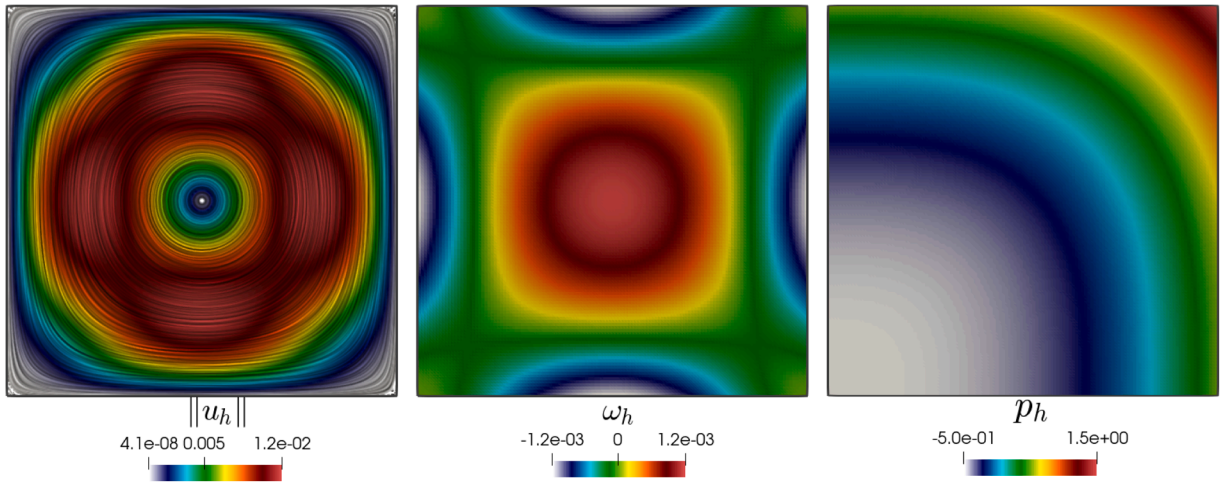
Fig. 1. Approximate velocity (line integral contours and magnitude), vorticity, and Bernoulli pressure profiles computed with the modified CR – \mathbb{P}_0 - \mathbb{P}_0 scheme, with kinematic viscosity \nu = 10^{-4} .
