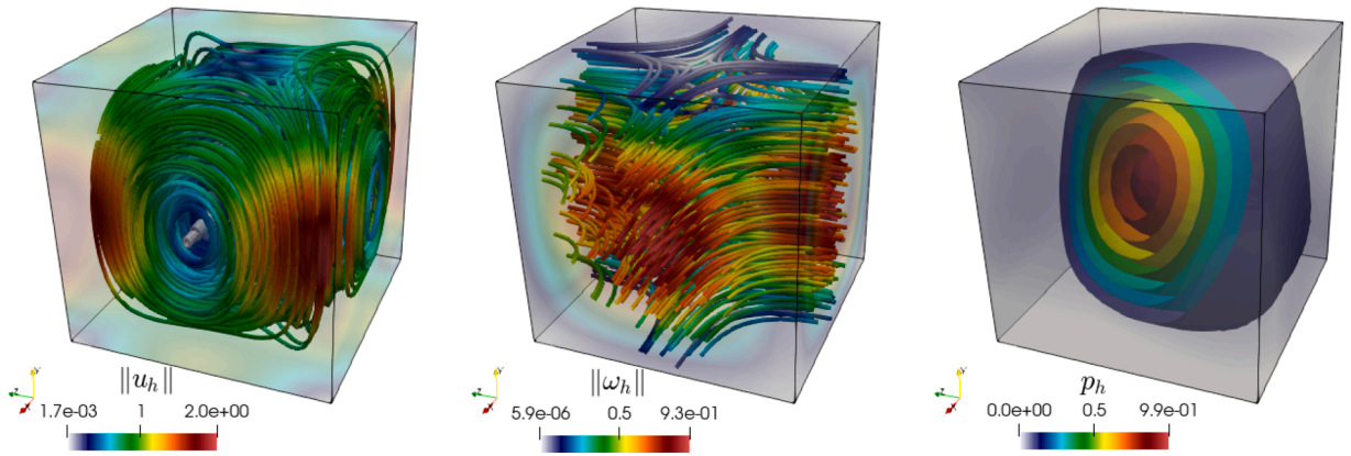
Fig. 2. Approximate velocity (streamlines), vorticity (streamlines), and Bernoulli pressure profiles on a mesh with h = 0.0383 , computed with the modified \text{CR} - \mathbb{P}_0 - \mathbb{P}_0 scheme (representing 241,153 DoFs), with kinematic viscosity \nu = 1 .
