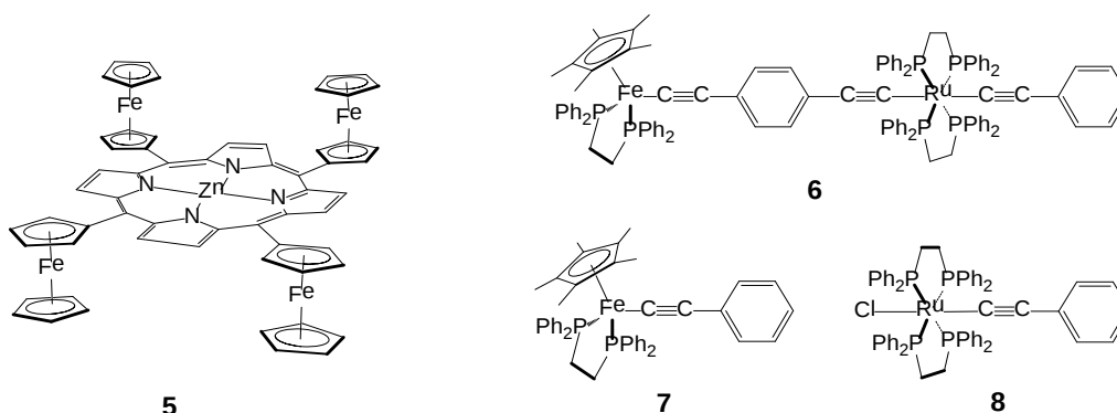
Scheme 3. Selected Compounds.
