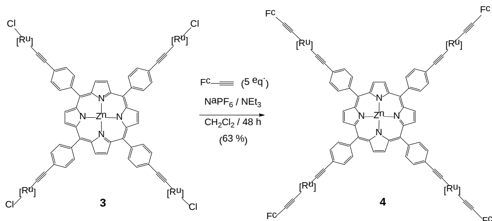
Scheme 2. Synthesis of 4 .
