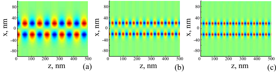
Fig. 3. Magnetic field distribution in lossless case for 40 nm slot waveguide for the free space wavelength \lambda = 465\text{nm} : (a) backward antisymmetric mode, (b) forward antisymmetric, and (c) symmetric modes.
