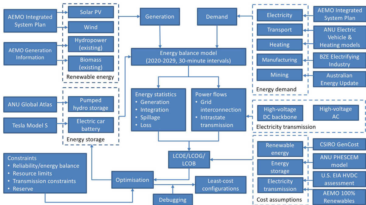
Fig. 3. Modelling framework. Acronyms and abbreviations: Australia Energy Market Operator (AEMO), Australian National University (ANU), Beyond Zero Emissions (BZE), Commonwealth Scientific and Industrial Research Organisation (CSIRO), U.S. Energy Information Administration (U.S. EIA).
