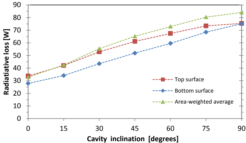
Fig. 5. Comparison of radiative loss values based on difference cavity temperature assumptions
