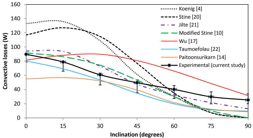
Fig. 6. Comparison of experimental data from current study to correlations cited in literature
