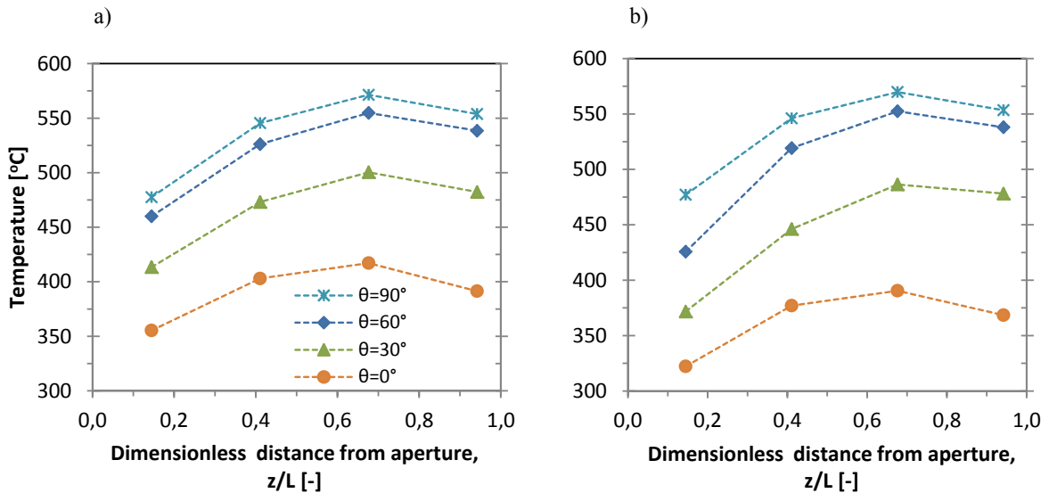
Fig. 4. Surface temperature distribution inside the cavity with AR=2 , q=4260\text{W/m}^2 : a) top surface. b) bottom surface.
