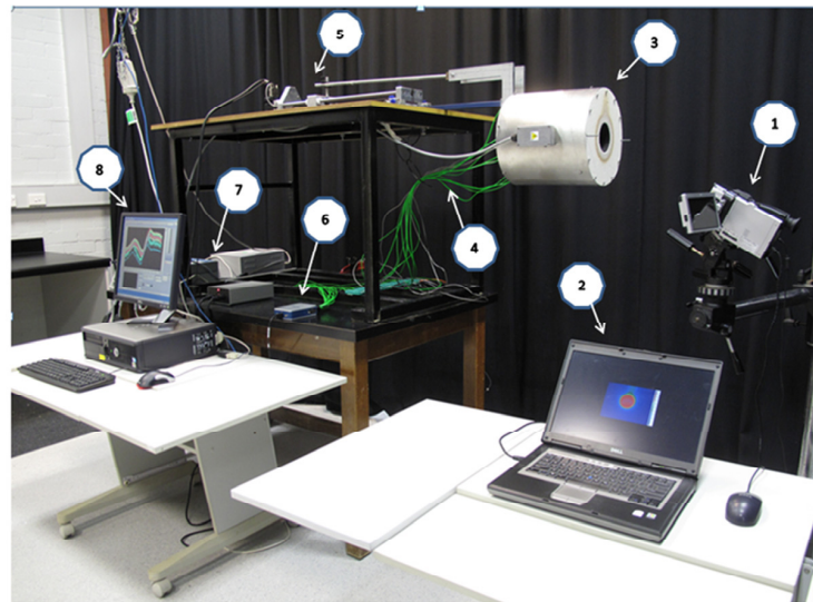
Fig. 2. Experimental setup for natural convection experiments – 1: Thermal camera, 2: Laptop, for thermal image acquisition, 3: Model cavity receiver, 4: Thermocouple connections, 5: Stepper motor, 6: Data logger, 7: Power controller, 8: PC used for data acquisition.
