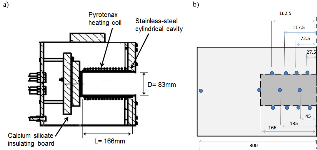
Fig. 3. Cross section of lab-scale cavity receiver, showing a) components of the receiver, b) thermocouple locations for cavity with AR=2
