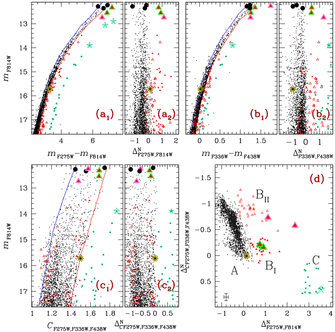
Figure 3. Zoom-in of the m_{F814W} versus m_{F275W} - m_{F814W} (panel a 1 ), m_{F814W} versus m_{F336W} - m_{F438W} CMD (panel b 1 ), and versus C_{F275W,F336W,F438W} diagrams around the RGB. The two fiducials used to verticalize the RGB are shown as thick red and blue lines (see text for details). The verticalized diagrams are plotted in panels (a 2 ), (b 2 ), and (c 2 ). Large black dots, red triangles, and aqua stars, respectively, mark the metal-poor, metal-intermediate, and metal-rich stars observed by Y14. Panel (d) shows the \Delta^N_{CF275W,F336W,F438W} versus \Delta^N_{F275W,F814W} diagram for RGB stars. RGB-A, RGB-B, and RGB-C stars are coloured black, red, and aqua, respectively. The mean error bar is shown in the lower-left corner. The magenta and green large triangles mark the metal-intermediate/Na-rich stars and metal-intermediate/Na-poor stars, respectively. The star analysed by Lardo et al. (2012) has been represented with a large asterisk.
