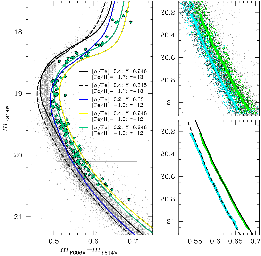
Figure 6. Left: m_{F814W} versus m_{F606W} - m_{F814W} CMD of M2, with five superimposed isochrones with the values of [Fe/H] , [alpha/Fe] , age, and Y listed in the figure inset. Aqua symbols highlight population C stars. Right: zoom-in of the same CMD shown in the left-hand panel around the MS (upper panel). A_{II} and A_{IV} stars, as defined in Fig. 5, are plotted with green and cyan points, respectively. The green and the cyan line are the fiducials of A_{II} and A_{IV} MSs. In the lower-right panel, we have superimposed the two metal-poor isochrones on the fiducials.
