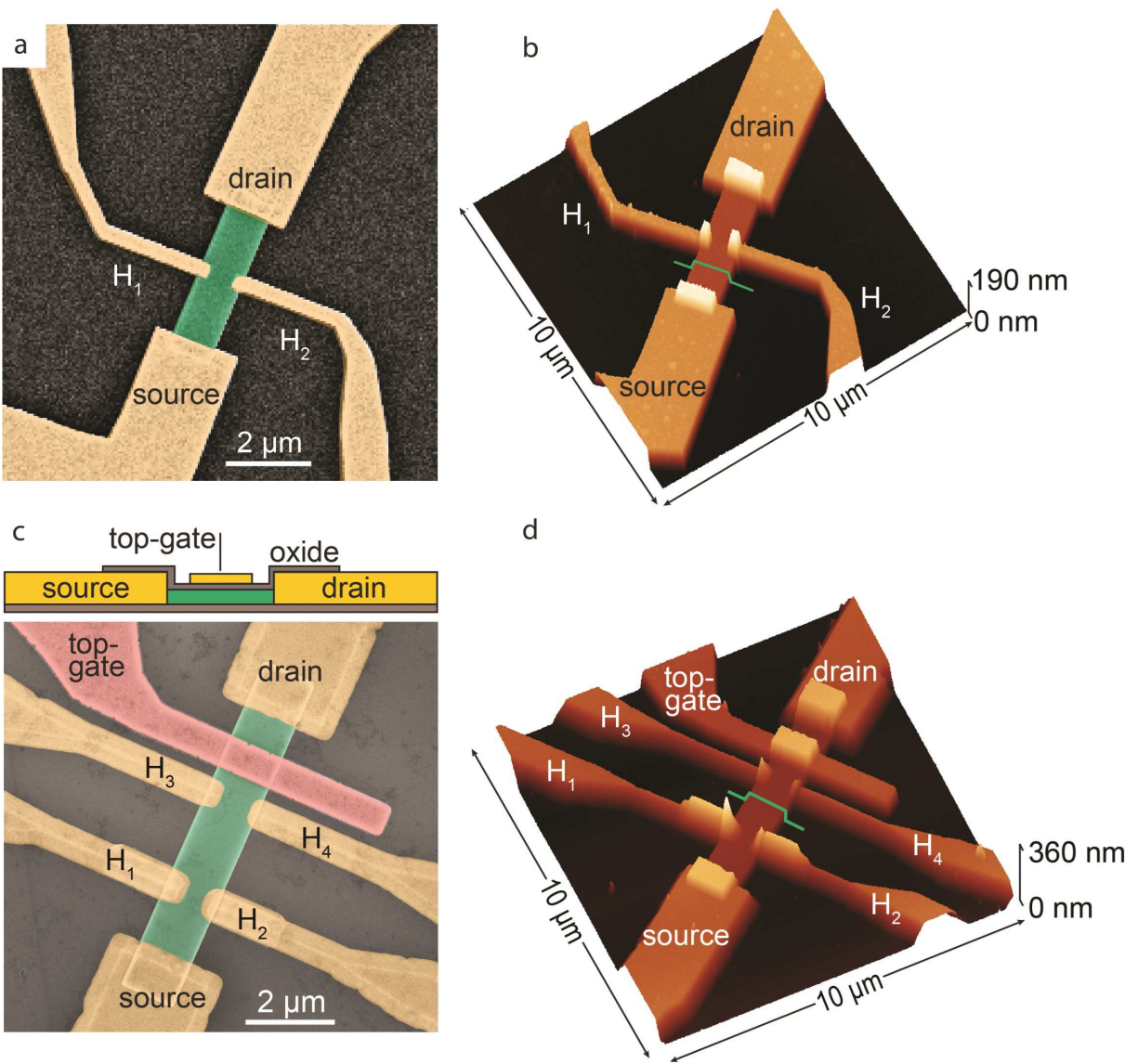
Figure 3: Fabrication of nanofin devices for Hall effect and local gating studies a false-color SEM and b AFM image of a device for Hall effect studies (Device 1) featuring a nanofin (green), source, drain and a pair of Hall contacts H_1 and H_2 (yellow). c Schematic and false-color SEM and d AFM image of a patterned top-gate device (Device 2) featuring nanofin (green), set of six contacts (yellow), and a \text{HfO}_2 insulated top-gate (red). The scale bars in a and c represent 2 \mu\text{m} . The green dotted lines in b and d indicate the locations of an AFM line-scan revealing nanofin thicknesses of 74 nm and 85 nm for the two devices, made from separate growths (see Supplementary Fig. S7).
