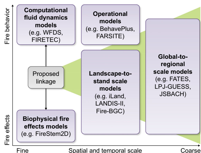
Fig. 1 Model classification according to scale and process representation. In this conceptual figure, we show the classification applied to different models of fire behavior and effects discussed in this review. We also highlight our proposed linkage between fine-scale computational fluid dynamics (CFD) and biophysical fire effects models.
