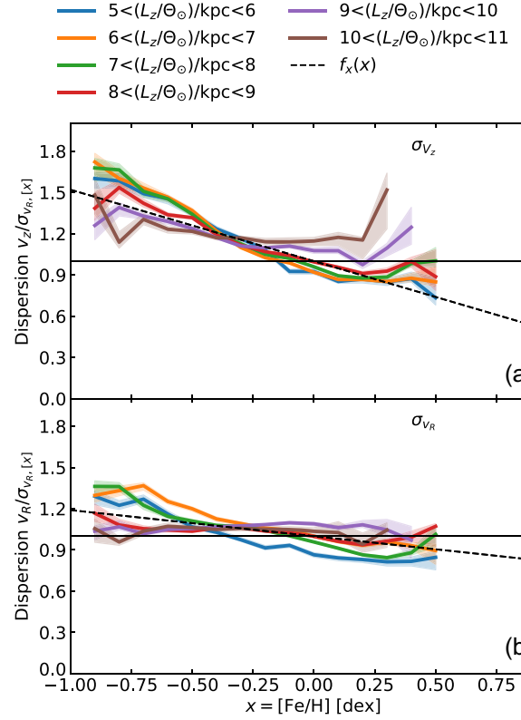
Figure 7. Velocity dispersion as a function of metallicity, [Fe/H], for stars lying in different angular momentum bins. The shaded region denotes the 16 and 84 percentile confidence interval. The curves are normalized to have unit dispersion at [Fe/H] = 0. The dependence on other independent variables ( L_z , age, and |z| ) have been divided out (see Section 3.2). The description of the panels and the data set used are same as in Fig. 3. The profiles show a mild variation with L_z , with the profiles becoming flatter with increase of L_z .
