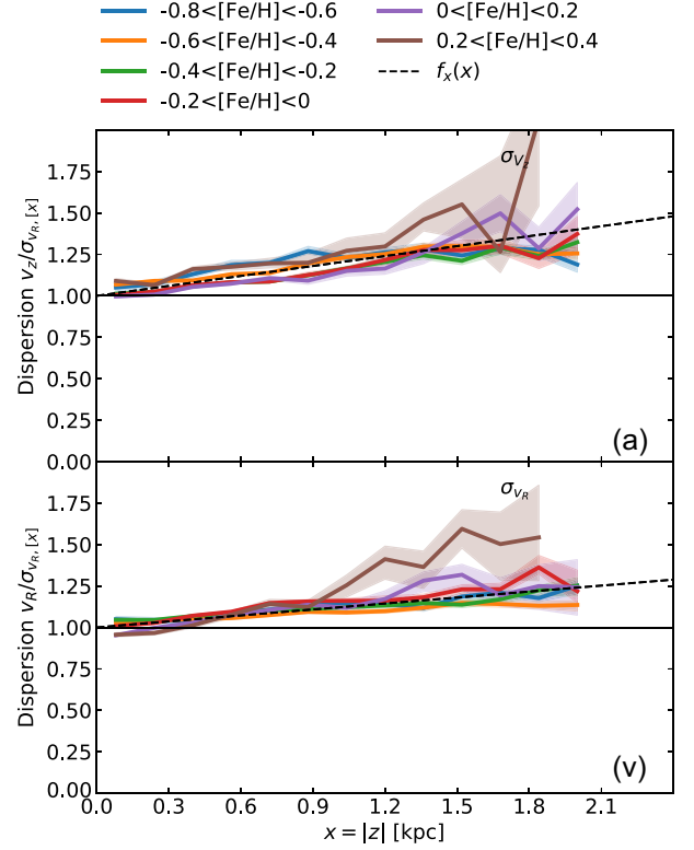
Figure 11. Same as Fig. 9 but for stars lying in different [\text{Fe}/\text{H}] bins. The relationship shows very little variation with [\text{Fe}/\text{H}] .
