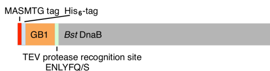
Figure S1. Bst DnaB expression construct used. The N-terminal fusions increased the molecular mass of the monomeric protein to 58.7 kDa. Due to the flexibility of the linker between GB1 domain and DnaB, this increase in molecular mass is not expected to influence the NMR spectrum of the hexamer very much.
