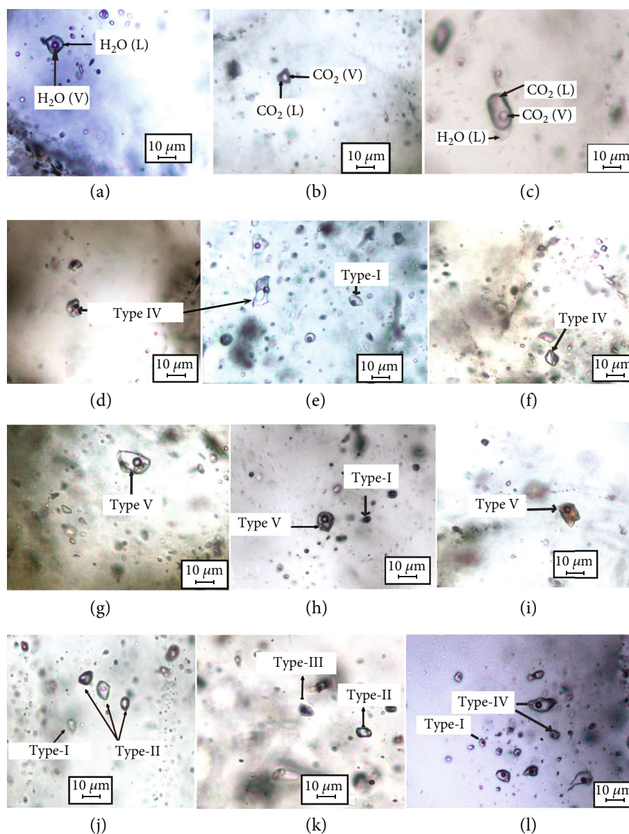
FIGURE 4: Fluid inclusion petrography. (a) Typical type I (aqueous L+V) inclusions as part of random three-dimensional network in the matrix of quartz in the BGQR system. (b) Type II inclusion in the usually observed size. (c) A typical type III inclusion as observed at room temperature, with high proportion of carbonic liquid. (d–f) Type IV inclusions (see text for details) with variable sizes and nature of solid phases. (g–i) Type V inclusions with variable sizes, number of moving objects within the inclusion cavity, and the color of the aqueous liquid (see text). (j) Occurrence of type I and II inclusions in close spatial association. (k) A rare instance of occurrence of type II and type III inclusions. (l) Representative of close spatial occurrence of type I and type IV inclusions observed only in samples of vein quartz in the reef (as depicted in Figure 2(g)).
