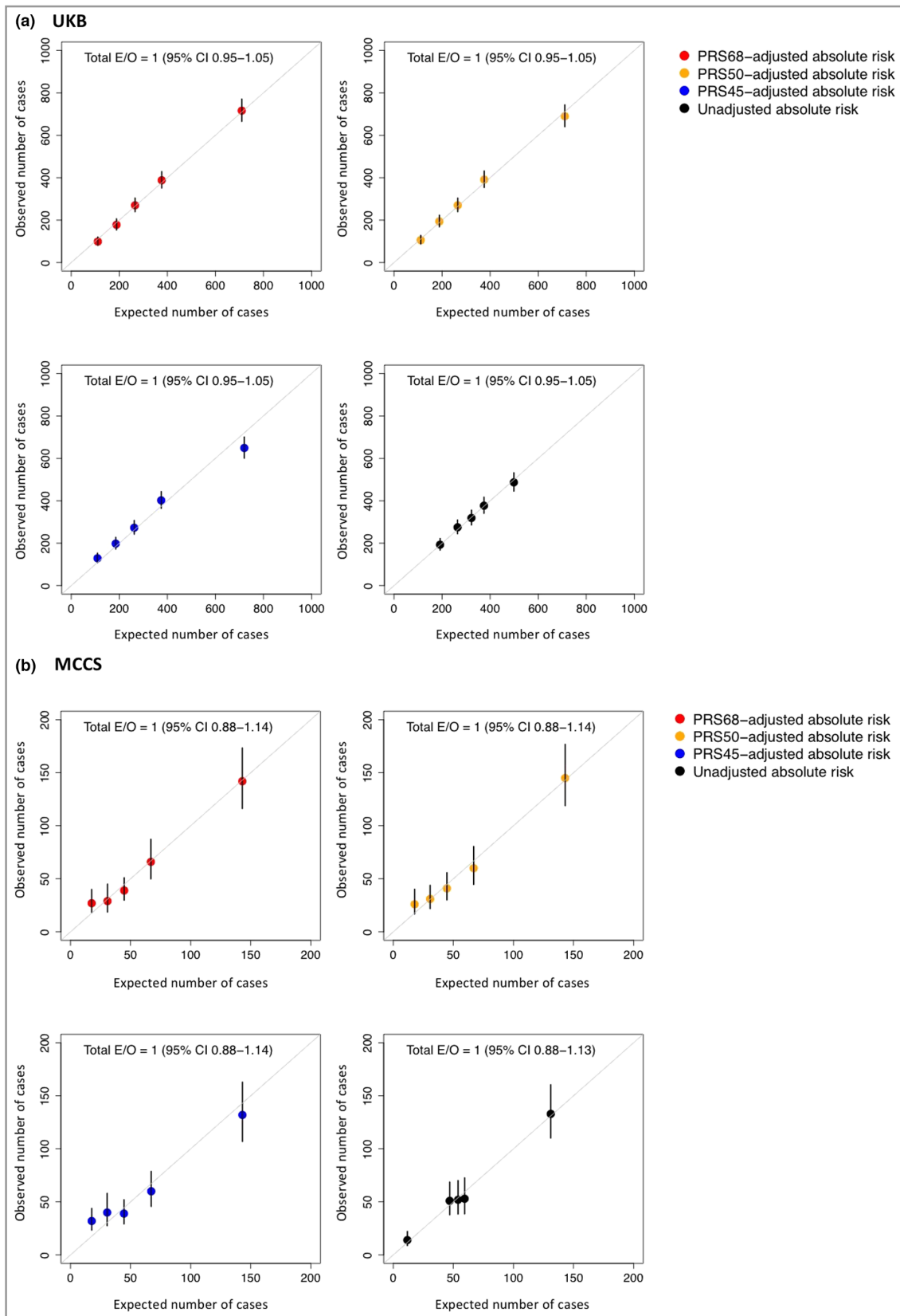
Figure 2 Calibration of absolute melanoma risks after rescaling to expected/observed (E/O) = 1 in (a) the UK Biobank (UKB) and (b) the Melbourne Collaborative Cohort Study (MCCS), by risk quintile. Bars show 95% confidence intervals (CIs).
