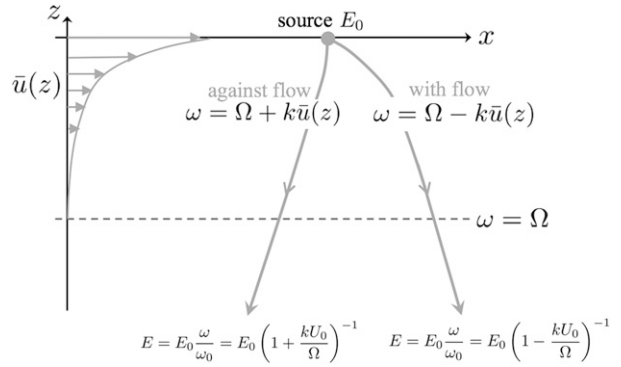
FIG. 11. Schematic of the amplification (decay) of wave energy in a mean shear flow \bar{u}(z) for waves propagating with (against) the flow, following Eliassen and Palm (1961); Yamanaka and Tanaka (1984); and Xie and Vanneste (2017), among others. The basic principle is that wave action A = E/\omega , where E is the energy and \omega the Eulerian frequency, is conserved so that wave energy scales with frequency. Parameter \Omega is the Lagrangian (intrinsic) frequency of the wave, and U_0 = \bar{u}(0) is the change in velocity seen by the wave. For small amplifications (e.g., 10%–20%, as seen in the present simulations), the fractional increase in energy is just kU_0/\Omega .
