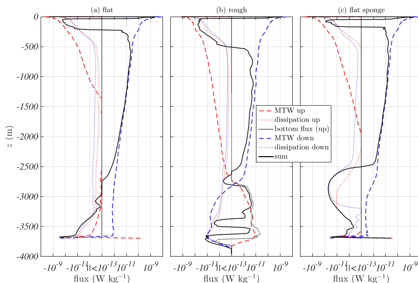
FIG. 4. Vertical profiles of the sources and sinks of wave energy ( W\ kg^{-1} ) for the three simulations: (a) flat (case A), (b) rough (case B), and (c) flat sponge (case C). The sum of all sources and sinks at a given depth is shown in black.
