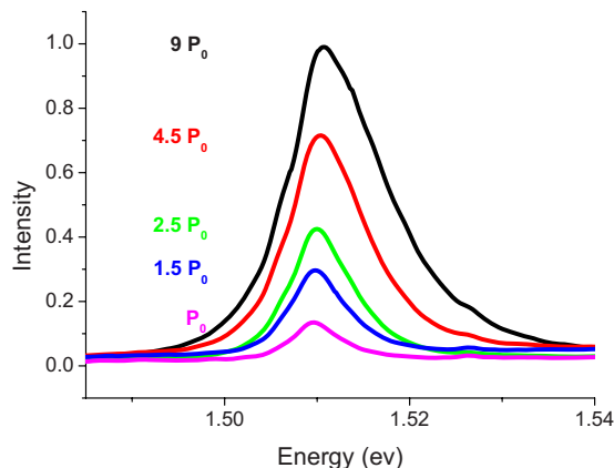
FIG. 2. (Color online) cw PL spectra as a function of power from single GaAs/AlGaAs NW (wire 2). P_0 \sim 30 \mu\text{W} .
