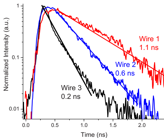
FIG. 3. (Color online) Low-power time decays accumulated at the peak emission energy (1.515 eV) from three single GaAs/AlGaAs core-shell NWs grown using the two-temperature technique.
