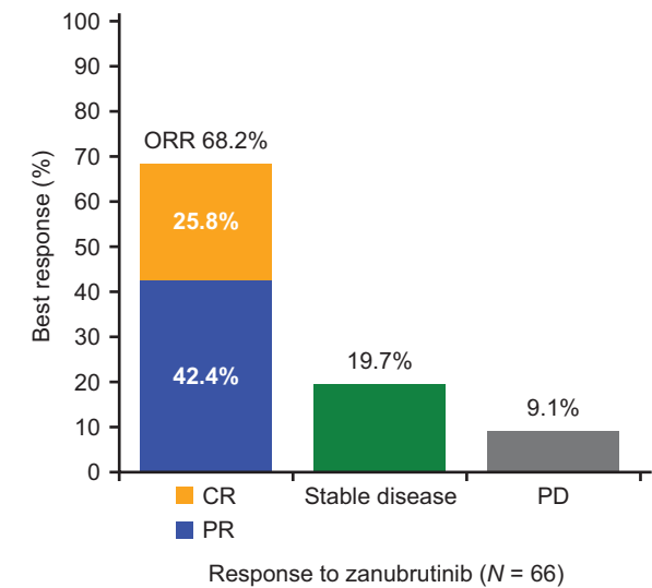
Figure 3. ORR per IRC assessment based on Lugano classification (15) for MZL patients in the MAGNOLIA study (BGB-3111-214).
