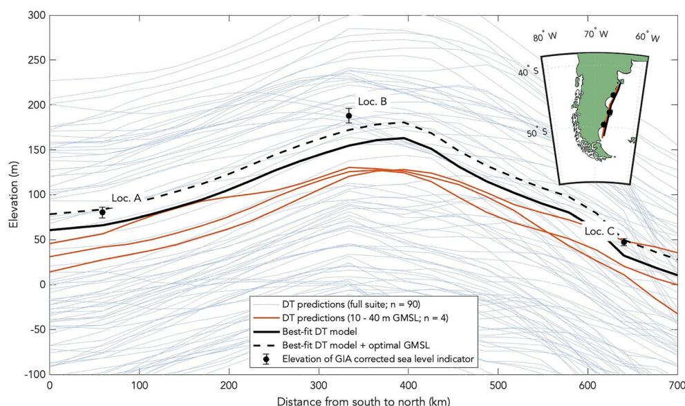
Figure 8. Great circle profiles of DT change across the Patagonian foreland from south to north through the three sea level indicator sites. GIA-corrected elevations are shown by black markers (uncertainties are 1\sigma ). Red profiles show DT change predictions that lead to global mean sea level (GMSL) estimates within 10–40 m. While these predictions correspond to more realistic GMSLs, many achieve poor fits to the GIA-corrected shoreline elevations. The best fitting model is shown in black and its associated sea level prediction including GMSL inference is shown as the black dashed line. Map indicates great circle paths of the preferred models.
