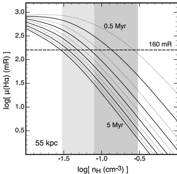
Figure 6. MAPPINGS IV time-dependent isochoric calculations of the change in H\alpha surface brightness after a Seyfert flare has occurred at the Galactic center ( D = 55 kpc, f_E = 0.1 ; Z = 0.1 Z_\odot ). The canonical Stream brightness (160 mR) is shown as a horizontal dashed line. The tracks plotted every 0.5 Myr show the relation between H\alpha and gas density at a fixed recombination time T_R . The associated look-back times (offset by the light crossing time) are shown in Table 1. The dark vertical band shows the range in n_H consistent with the known cloud properties; the lighter band is marginally consistent.
