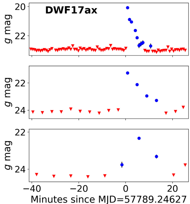
Figure 2. Light curves of the fast transient candidate labelled DWF17ax (whose discovery images are shown in Fig. 3) obtained with individual 20 s exposures ( top ) and by stacking sets of five ( centre ) and nine ( bottom ) fast-cadence images. Red triangles indicate 5\sigma upper limits.
