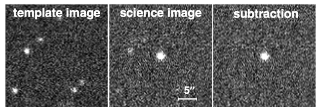
Figure 3. Example of detection ‘postage-stamp’ images. The eFTC (in this case DWF17ax) is present in the science image ( centre ) and is not present at the same coordinates in the deeper template images ( left ). The image subtraction between science and template images leaves a bright, PSF-shaped residual brighter than the background ( right ). The light curve of DWF17ax is shown in Fig. 2.
