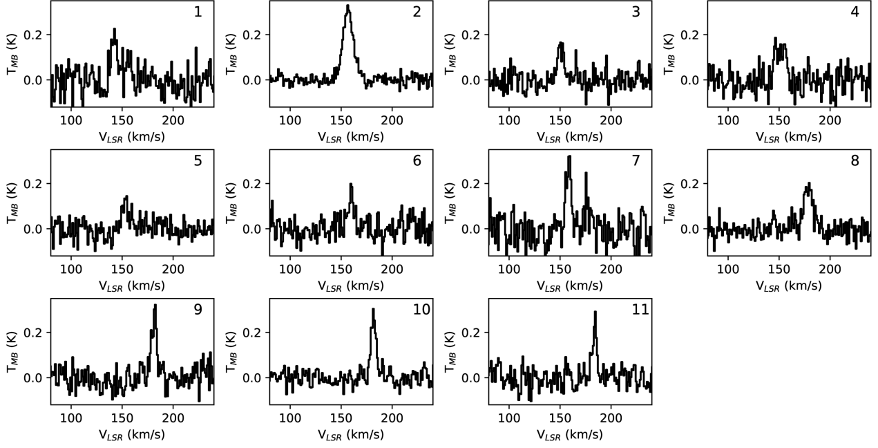
Fig. 3. Coadded average ^{12}\text{CO} J=1–0 spectra for each molecular clump in MW-C21 based on the 3 dimensional mask array.
