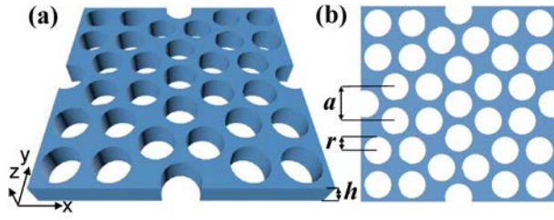
Fig. 1. (a) 3D schematic and (b) 2D top view of the silicon PQC structure with supercell simulation range.
