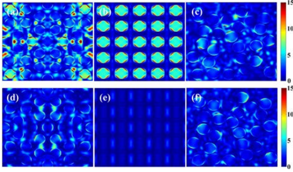
Fig. 3. E-field intensity distributions (azimuth angle \phi = 0^\circ ) in (a) PQC, (b) Ordered and (c) Random structures at \lambda = 624.6 nm. E-field intensity distributions in (d) PQC, (e) Ordered and (f) Random structures at \lambda = 662.4 nm.
