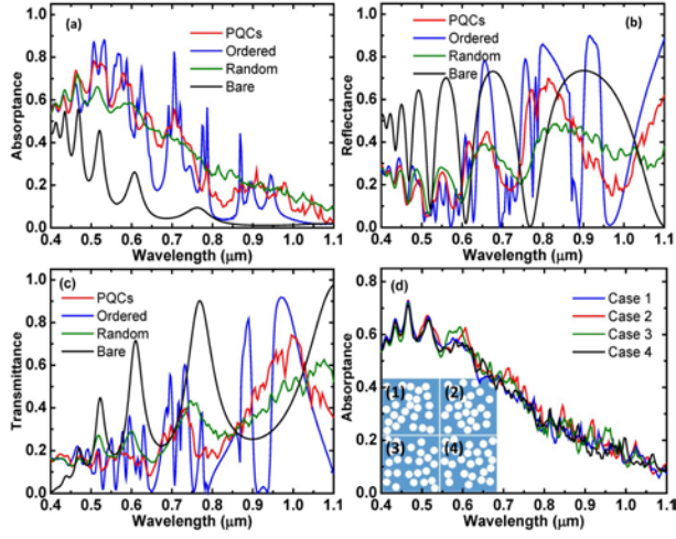
Fig. 2. (a) Absorbance, (b) reflectance, and (c) transmittance of PQC, Ordered and Random structures, and (d) absorbance of four different Random structures.
