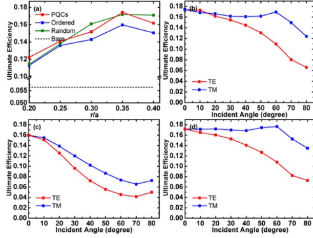
Fig. 4. (a) Ultimate efficiency of the PQC, Ordered and Random structures for different ratio of radius of NH to lattice constant, r/a . Angular response and polarization dependence of the ultimate efficiency of the (b) optimized PQC, (c) Ordered and (d) Random structures.
