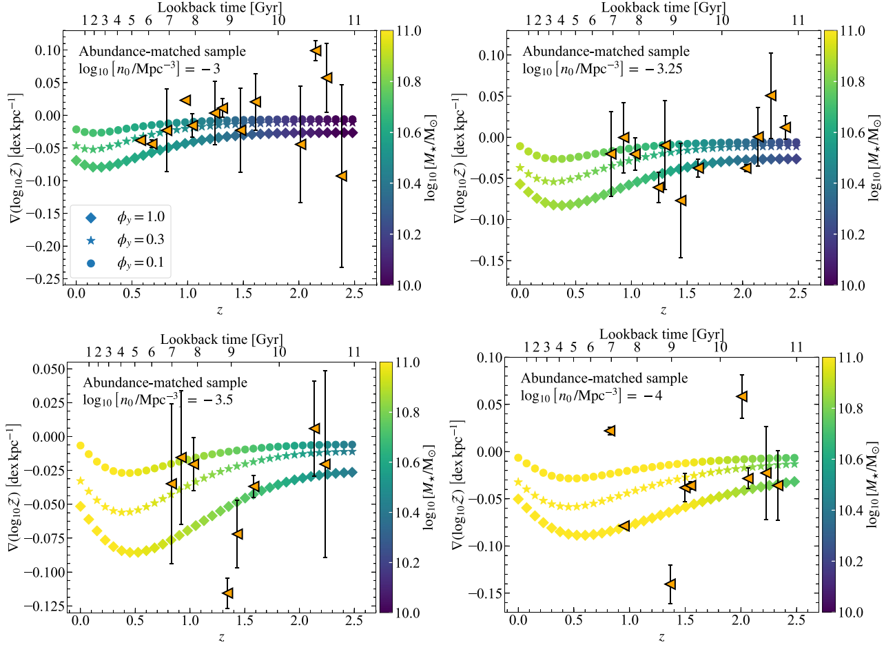
Figure 12. Trends in metallicity gradients as a function of z (and look back time) for four different abundance-matched galaxy samples, given a fixed comoving number density of galaxies, n_0 , colour-coded by M_* . Abundance matching leads to the selection of more massive galaxies at lower redshifts and can be used to collectively study gradients in local spirals and their high- z progenitors. The orange data points reflect mean gradients for a constructed abundance-matched sample from available observations, which are the same as that reported in Fig. 11, with error bars representing the scatter within the data. There is considerable scatter in the data, and the sample is not entirely robust, given the ex post facto construction. None the less, the model matches the observations reasonably well.
