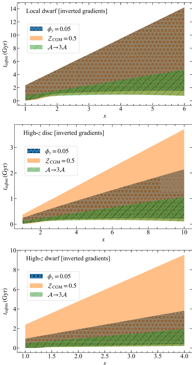
Figure 16. Metallicity equilibration time-scale t_{\text{eqbm}} as a function of x in galaxies with inverted gradients. The first panel represents t_{\text{eqbm}} in local dwarfs. The second panel on high- z discs is identical to the class of high- z galaxies we discuss in Section 3.3. The third panel plots t_{\text{eqbm}} in the case of high- z dwarfs that we create by combining the fiducial parameters for local dwarfs and high- z galaxies (see Section 5.2.3 for details). The colours correspond to the different ways that can give rise to an inverted gradient in a galaxy: reduction in metal yield due to high preferential metal ejection ( \phi_y = 0.05 ), enrichment of the CGM due to fountains or metal-rich flows ( Z_{\text{CGM}} = 0.5 ), and excessive cosmic accretion ( \mathcal{A} \rightarrow 3\mathcal{A} ). The scatter in the model is due to c_1 . This plot shows that inverted metallicity gradients may or may not be in equilibrium.
