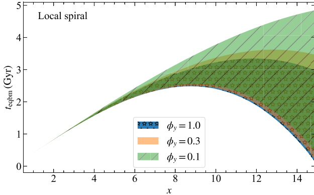
Figure 1. Metallicity equilibration time, t_{\text{eqbm}} , plotted as a function of the dimensionless radius x for three different values of the yield reduction factor, \phi_y , for a fiducial local spiral galaxy (see equation 19). Here, x = r/r_0 , where r_0 = 1 kpc. The shaded bands correspond to solutions that cover all allowed values of the constant of integration c_1 in the solution to the metallicity equation (see Section 2.3). Since, t_{\text{eqbm}} is substantially smaller than the Hubble time t_{\text{H}(0)} and comparable to the molecular gas depletion time t_{\text{dep}, \text{H}_2} , metallicity gradients in local spirals are in equilibrium.
