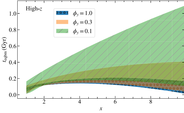
Figure 7. Same as Fig. 1, but for high- z galaxies. The corresponding equilibrium metallicity gradients are plotted in Fig. 8.
