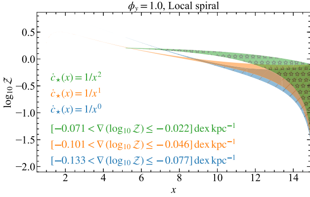
Figure A1. Same as Fig. 2 but with different functional forms for cosmic accretion, namely, \dot{c}_*(x) = 1/x^2 (the one we use in the main text), 1/x , and 1 , respectively. Flatter cosmic accretion profiles make the gradients steeper (within a factor of 2).
