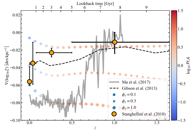
Figure B1. Same as Fig. 10, but with \sigma_g(z) reduced by a factor of 1+z as compared to equation (53) (see Appendix B for a discussion).
