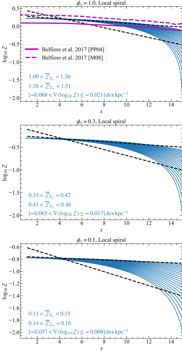
Figure 2. Metallicity ( Z = Z/Z_\odot ; blue lines) as a function of dimensionless radius ( x = r/r_0 with r_0 = 1 kpc) produced by the model for a fiducial local spiral galaxy with input parameters listed in Tables 1 and 2, for different values of the yield reduction factor, \phi_y . The analytic solution to the metallicity evolution equation is given by equation (41). The slope of the linear fit to the model gradients between x = 1 – 15 (black, dashed lines) gives the metallicity gradient that can be compared against simulations and observations. The blue coloured curves show the acceptable parameter space of the gradients based on the constraints on the constant of integration, c_1 , using the boundary conditions criteria described in Section 2.3. The metallicity at the inner edge of the disc (referred to as the central metallicity in the text), Z_{r_0} , is set by the balance between source and accretion for local spirals (see equation 48). \overline{Z}_{\Sigma_g} and \overline{Z}_{\Sigma_\star} represent the range of mass-weighted and SFR-weighted mean equilibrium metallicities produced by the solution, respectively (see equation 45). We expect \phi_y closer to unity for local spirals, implying that metals in these galaxies are well mixed with the ISM before they are ejected. Finally, in the top panel, we overplot the average metallicity profiles observed in local spirals in the MaNGA survey by Belfiore et al. (2017) using the PP04 (Pettini & Pagel 2004) and M08 (Maiolino et al. 2008) calibrations, adjusting the normalization to overlap with the model profiles.
