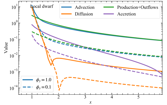
Figure 6. Same as Fig. 3, but for local dwarfs. The dominant terms that set the gradients in local dwarfs are advection and diffusion (in the inner disc) and source and advection (in the outer disc).
