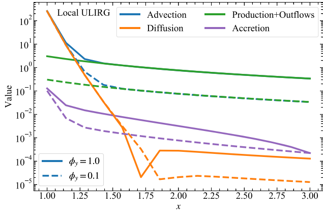
Figure 15. Same as Fig. 3, but for ULIRGs, which are known to be major mergers. The non-equilibrium metallicity distribution is set by advection of gas due to tidal inflows during a merger.
