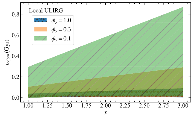
Figure 14. Same as Fig. 1, but for local ultraluminous infrared galaxies (ULIRGs). Here, t_{\text{eqbm}} \sim t_{\text{merge}} , where the latter is the merger time-scale of the order of \sim 0.3 - 1 Gyr as seen in models (Jiang et al. 2008; Torrey et al. 2012). Thus, the metallicity gradients may not be in equilibrium throughout the merger process. In such a case, our equilibrium model for metallicity gradients cannot be applied to local ULIRGs, and the observed gradients, if any, are transient and subject to change as the merger progresses in line with observations (Rupke, Kewley & Chien 2010b; Rich et al. 2012).
