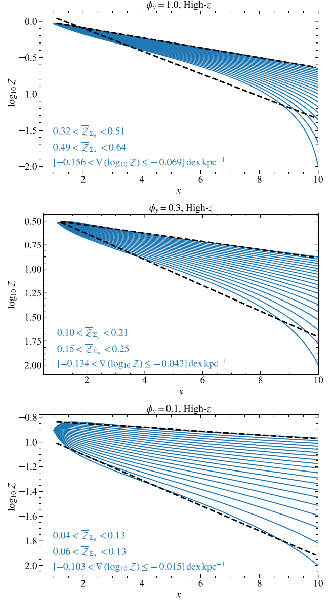
Figure 8. Same as Fig. 2, but for high- z galaxies. Here, \mathcal{Z}_{r_0} is set by the balance between diffusion and advection.
