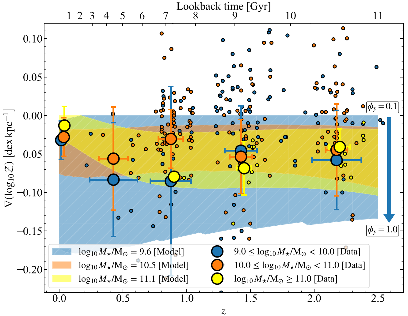
Figure 11. Trends in metallicity gradients as a function of redshift and look back time. Coloured markers represent individual galaxies within the three M_* bins as shown in the legend, with bigger markers representing binned averages of non-positive gradients across different redshift bins and error bars representing the scatter in the data within each redshift bin. The averages at z = 0 are taken from local surveys (Sánchez et al. 2014; Sánchez-Menguiano et al. 2016; Belfiore et al. 2017; Mingozzi et al. 2020). The high-redshift compilation data are taken from Queyrel et al. (2012), Swinbank et al. (2012), Stott et al. (2014), Leethochawalit et al. (2016), Wuyts et al. (2016), Molina et al. (2017), Carton et al. (2018), Förster Schreiber et al. (2018), Wang et al. (2020), and Curti et al. (2020) and are inhomogeneous, with systematic issues within the different measurements (see Section 4.2). The coloured bands represent models at three M_* values, with the spread resulting from different yield reduction factors \phi_y , as marked by the arrow besides the shaded region. This spread in the model is largest for the low-mass galaxies. While the general trend of mild evolution of gradients across redshift holds true, the models uncover the underlying variations due to galaxies transitioning from advection- to accretion-dominated regimes between z = 2.5 and 0, as is visible in the binned data averages. Some data points lie outside the range of the plot, and we do not include those for the purposes of studying the average trends of the data with the model.
