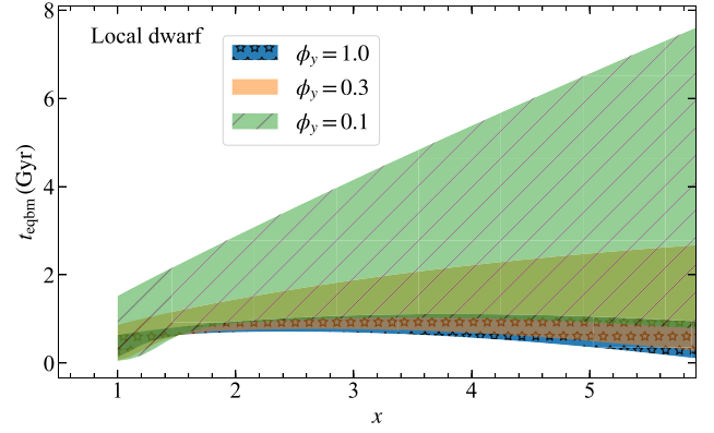
Figure 4. Same as Fig. 1 but for local dwarfs. Here, t_{\text{eqbm}} < t_{\text{H}(0)} , implying that the metallicity gradients in local dwarfs are also in equilibrium, even in the case of low \phi_y (see the text for a discussion on t_{\text{dep,H}_2} for local dwarfs). The corresponding metallicity gradients are plotted in Fig. 5.
