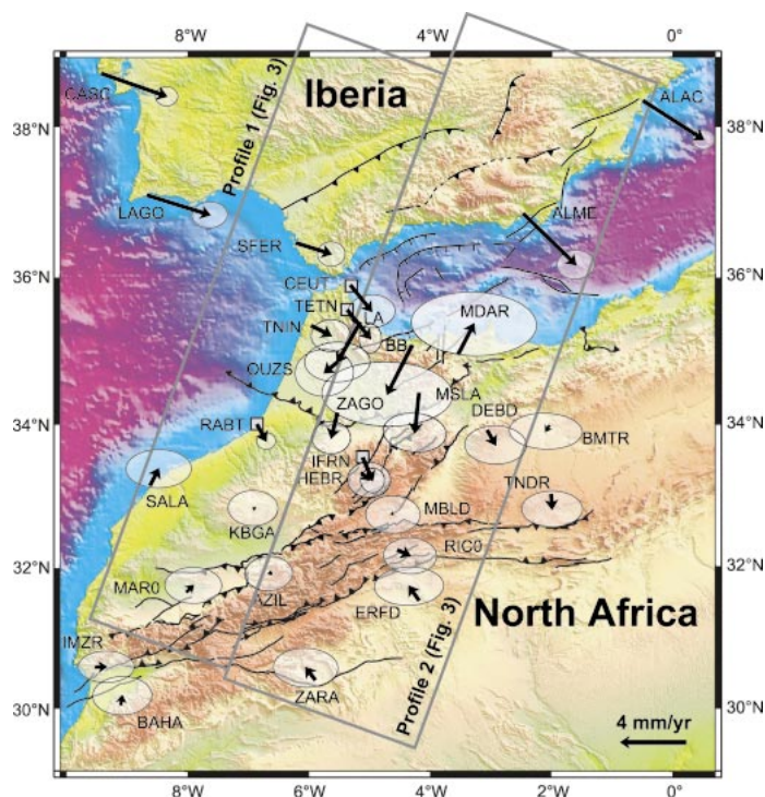
Figure 2. Map showing GPS-derived site velocities and 95% confidence ellipses relative to Africa for sites in Morocco and adjacent Iberia (GPS stations are identified by four letters; BB—BBFH; LA—LAOU). Continuously recording GPS (CGPS) stations in northwestern Africa are indicated by squares. Gray boxes show the orientation and width of profiles 1 and 2 in Figure 3; the profiles go farther north to southern France. Base map as in Figure 1.
