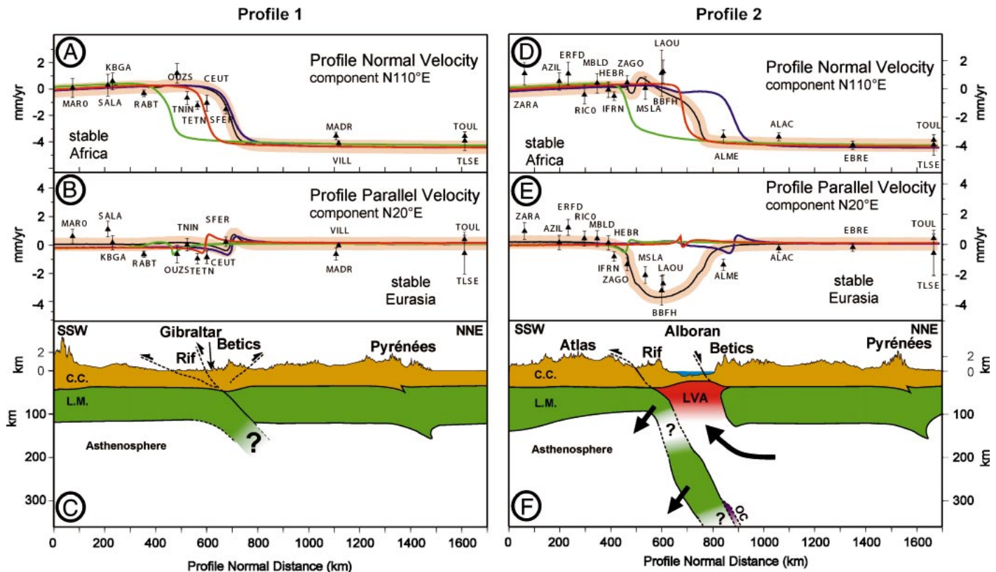
Figure 3. Profile 1 and profile 2 (locations in Fig. 2). A and D: Component of velocities and 1\sigma uncertainties along the direction of plate motion (normal to profile). B and E: Component of velocities and 1\sigma uncertainties parallel to the direction of plate motion (i.e., parallel to profiles). Interseismic deformation predicted by elastic block models is shown for three main hypothesized plate boundaries (red—Klitgord and Schouten, 1986; green—Bird, 2003; blue—Gutscher, 2004; see Fig. 1 for geometry). Thick pink line with thin black line in the center is for a model with a central Rif block (see Fig. 4 for geometry). C and F: Topography and interpretative cross section along profiles 1 and 2. LVA—low-velocity and high-attenuation anomaly (Calvert et al., 2000; Seber et al., 1996); CC—continental crust; LM—lithospheric mantle; OC—oceanic crust.
