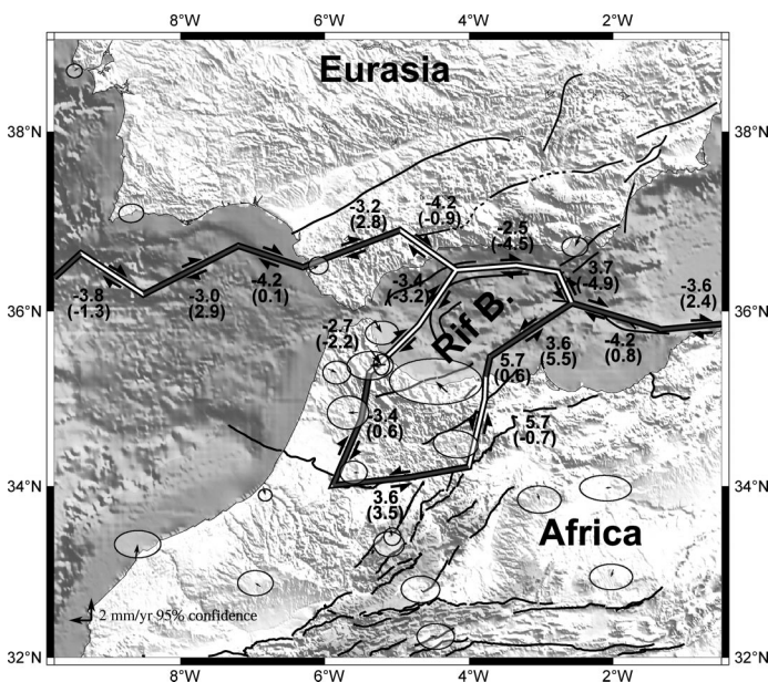
Figure 4. Map showing elastic block model for Africa-Eurasia plate boundary in western Mediterranean, and GPS residual velocities and 95% confidence ellipses for our preferred model. Numbers show strike-slip and fault-normal average slip rates along each segment in mm/yr (fault-normal component in parentheses; negative for left-lateral and extension). Gray modeled faults indicate segments with fault-normal shortening. Formal uncertainties on model slip rates are ~1 mm/yr. Rif B.—Rif block.
