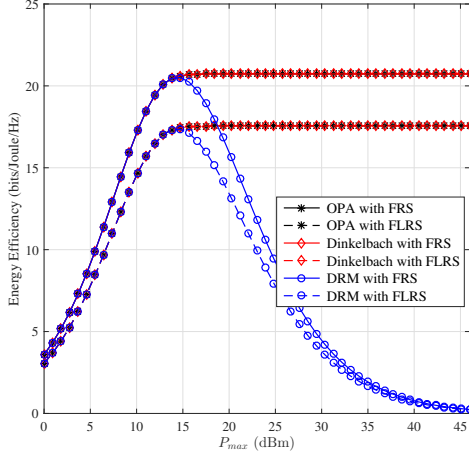
Fig. 7: Energy efficiency vs. maximum transmit power with different power allocation methods and relay selection schemes, where P_c = 10 dBm and \sigma^2 = -125 dBm.
