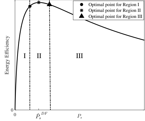
Fig. 3: Energy efficiency vs. transmit power within feasible regions.
