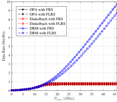
Fig. 8: Data rate vs. maximum transmit power with different power allocation methods and relay selection schemes, where P_c = 10 dBm and \sigma^2 = -125 dBm.
