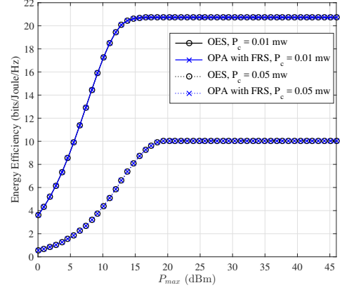
Fig. 9: Comparison of OES and OPA with FRS, where \sigma^2 = -125 dBm.
