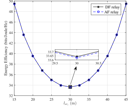
Fig. 5: Energy efficiency vs. distance between the source node and the relay in both DF and AF relay cases, where P_c = 10 dBm, P_{max} = 46 dBm, and \sigma^2 = -125 dBm.
