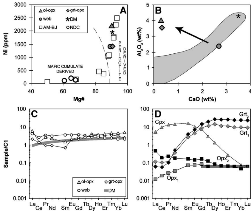
Fig. 4. A: Mg# versus Ni (in ppm) plot of orthopyroxenites (this work) and of harzburgites, garnet–orthopyroxenites, garnet–websterites, garnet–clinopyroxenites and eclogites from Maowu layered intrusion [35]. For comparison, Depleted Mantle [39] and mafic rocks data from the North Dabie Complex [50] are also reported. The shaded line represents the possible transition from cumulates to peridotites. B: CaO versus Al 2 O 3 wt.% concentrations of the studied samples and of Depleted Mantle. The compositional variation of orogenic, ophiolitic and abyssal peridotites is also showed in the grey field (from Bodinier and Godard [40]). The black solid arrow represents the relative enrichment in Al 2 O 3 with decreasing CaO of Maowu orthopyroxenites, compared with the grey area representing a peridotite depletion trend starting from the composition of Depleted Mantle [39]. C: Chondrite (C1) [51] normalised bulk-rock REE patterns are compared with Depleted Mantle (grey line) from Salters and Stracke [39]. D: Chondrite (C1) [51] normalised REE patterns of rock-forming minerals. Concentrations of each mineral phase are average of 5 representative analyses. The grey transparent line represents the detection limits for HREE. Mineral abbreviations after Bucher and Frey [49]; grt–opx = garnet-rich orthopyroxenite; web = websterite; ol–opx = orthopyroxenite with relict olivine; DM = Depleted Mantle; AM–BJ = mafic and ultramafic samples from Jahn et al. [35]; NDC = North Dabie Complex eclogites from Malaspina et al. [50].
