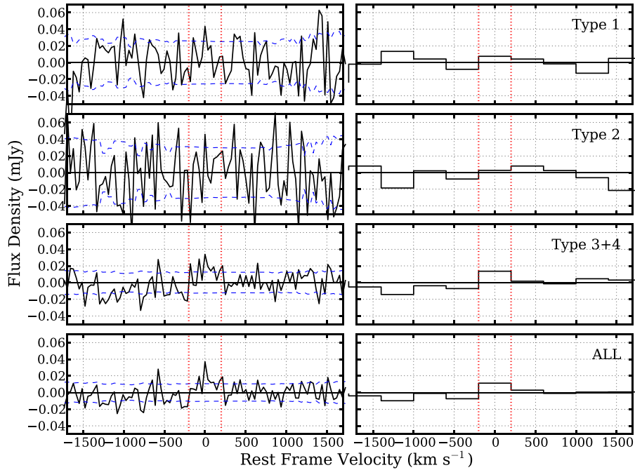
Figure 9. Stacked H I spectra of galaxies in each subgroup (left panels). The right panels show the re-binned stacked spectra with a velocity width of 500 km s -1 (the vertical dotted lines). The horizontal dashed line in each left panel is the 1 \sigma error of the stacked spectrum.
