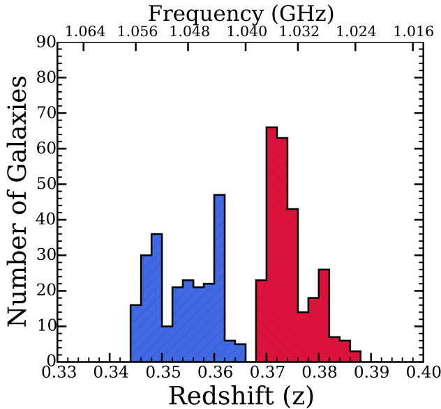
Figure 8. The redshift distribution of the COSMOS sample observed by the GMRT. Blue and red hatched areas are galaxies that lie in the upper and lower sidebands, respectively.
