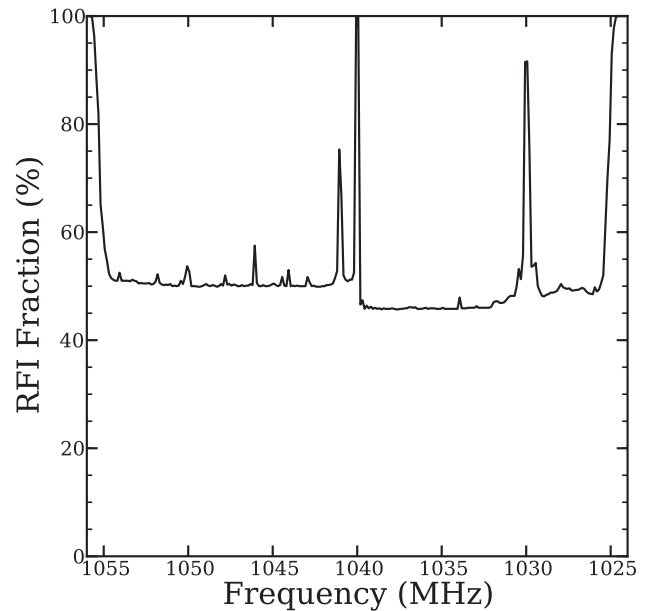
Figure 6. The fraction of flagged data after all data-reduction procedures.
