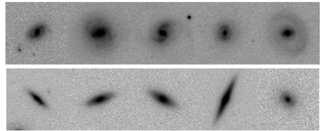
Figure 4. HST cutout images of blue early-type (upper row) and red spiral (lower row) examples. The size of each thumbnail image is 6 \times 6 arcsec 2 . The images were obtained using the G10/COSMOS image-cutout tool.
