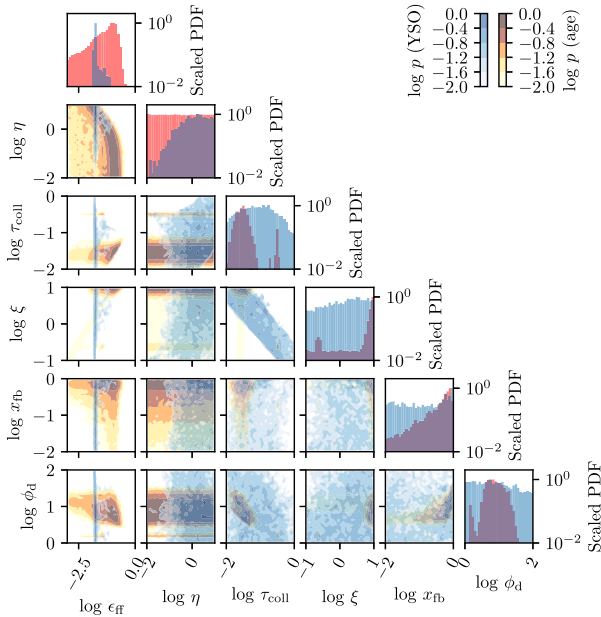
Figure 5. Same as Fig. 4, but showing the GCD model and its dimensionless parameters. Note that we show x_{\text{fb}} = t_{\text{fb}}/t_{\text{coll}} rather than \tau_{\text{fb}} = t_{\text{fb}}/t_{\text{sf}} , because the former quantity is more helpful for the discussion that follows.
