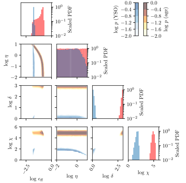
Figure 6. Same as Fig. 4, but showing the IE model and its dimensionless parameters.
