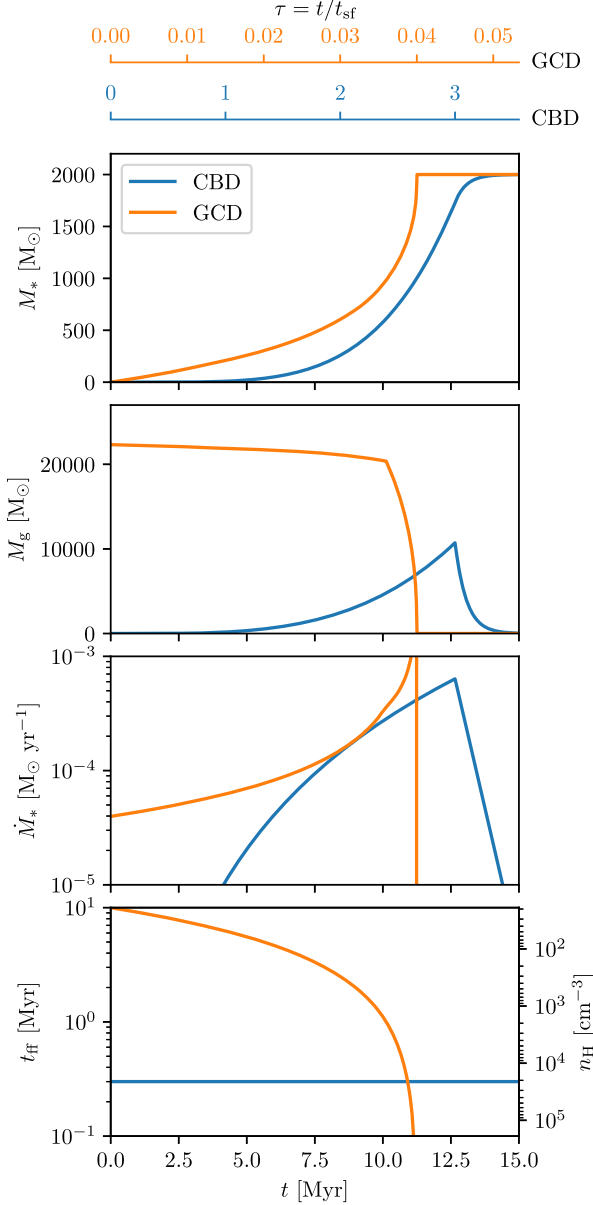
Figure 7. Example histories of stellar mass, gas mass, SFR, and free-fall time / density for the two best-fitting models, CBD and GCD, scaled to mass and time-scales typical of the ATLASGAL sample; the exact parameters used to construct these models are described in Section 3.3. The right axis in the bottom panel shows number density of H nuclei, computed assuming a mean mass of 1.4m_{\text{H}} per H nucleus. The bottom horizontal axis shows physical time in Myr, while the top two axes show dimensionless time \tau = t/t_{\text{sf}} ; this is different for the CBD and GCD models because the star formation time-scale t_{\text{sf}} is different in the two models.
