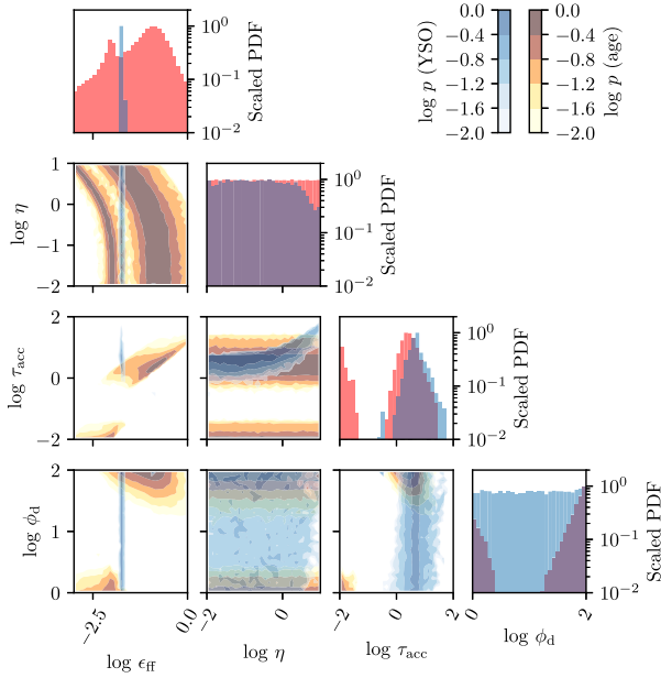
Figure 4. Corner plot showing the posterior PDF for the dimensionless parameters of the CBD model ( \epsilon_{\text{ff}} , \eta , \tau_{\text{acc}} , and \phi_d ), derived using the distribution of stellar ages in NGC 6530 (red colours) and the counts of YSOs in ATLASGAL clumps (blue colours). In the panels on the bottom left corner, contours show 2D marginal posterior PDFs for each combination of variables, as indicated on the axes. Histograms along the central diagonal show 1D marginal posterior PDFs for each variable. PDFs in all panels are scaled so that the maximum is unity.
