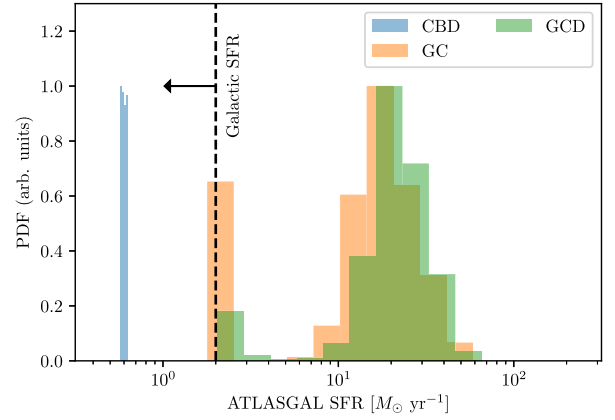
Figure 8. Histograms of predicted SFRs for the gas clumps in the ATLASGAL catalogue, using the CBD, GC, and GCD models with parameters constrained by fitting to the stellar age distribution in young clusters and the number of YSOs per unit gas mass in the ATLASGAL sample. All histograms have been normalized to have a maximum of unity for ease of comparison. The vertical dashed line marks the total SFR of the Milky Way (Chomiuk & Povich 2011); values to the left of this line, indicated by the arrow, are consistent with the total Galactic SFR, while values to the right of it are inconsistent.
