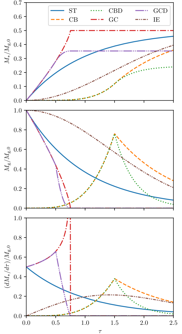
Figure 1. Example evolutionary histories of stellar mass (top), gas mass (middle), and SFR (bottom) for each of the models discussed in the paper (as indicated in the legend). For the purposes of this plot, we use \eta = 1 in all models. For CB and CBD, we use \tau_{\text{acc}} = 1.5 and p = 3 , for CBD and GCD we use \eta_d = 5 , for GC we use \xi = 1 and \tau_{\text{coll}} = 0.75 , for GCD we use \xi = 1 , \tau_{\text{coll}} = 0.75 , and \tau_{\text{fb}} = 0.5 , and for IE we use \chi = 0.5 and \delta = 1 . See main text for definitions of the various parameters.
