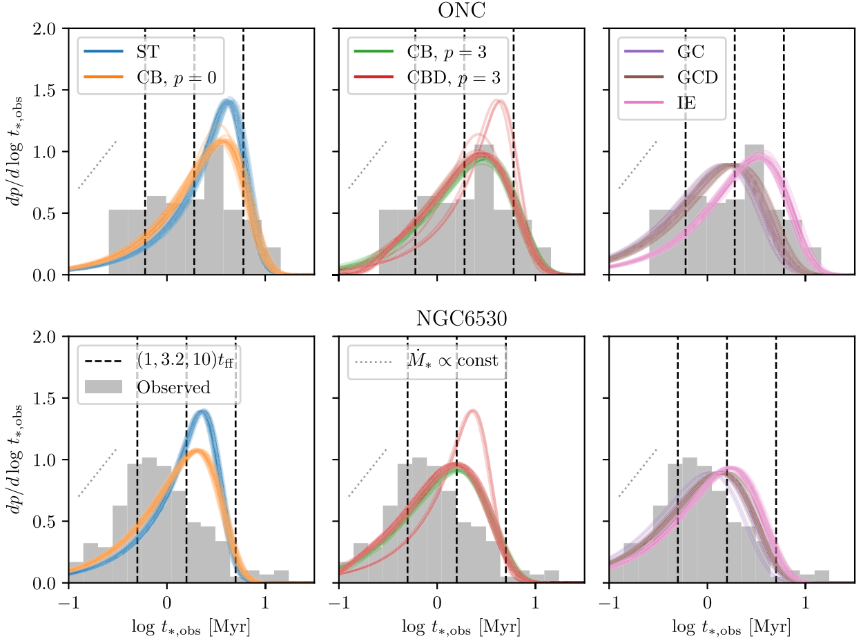
Figure 2. Distribution of observed stellar ages dp/d\log t_{*,\text{obs}} in the ONC (top) and NGC 6530 (bottom). In all panels, the coloured lines represent 20 random samples from the final iteration of the MCMC for each of the models, as indicated in the legend. Grey histograms show the observed distribution, and are the same in every panel. The dashed vertical lines indicate 1, 3.2, and 10\times the observed free-fall time, as indicated. The dotted grey lines, which we provide to guide the eye, are lines of slope unity, which, given the logarithmic age bins, corresponds to a constant SFR.
